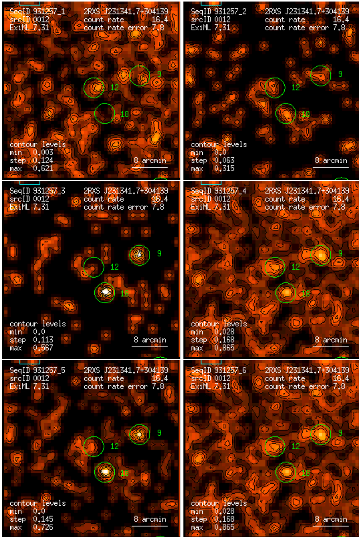
Figure 12: RASS 931257: detection 0012: band rate images, Gaussian filter: (1) PSPC channels 11 – 41, (2) 52 – 90, (3) 91 – 201, (4) 11 – 235, (5) 52 – 201, (6) 11 – 201. Broad band rates in counts/ks. Band rate contour levels in counts/ks/arcmin 2 .
