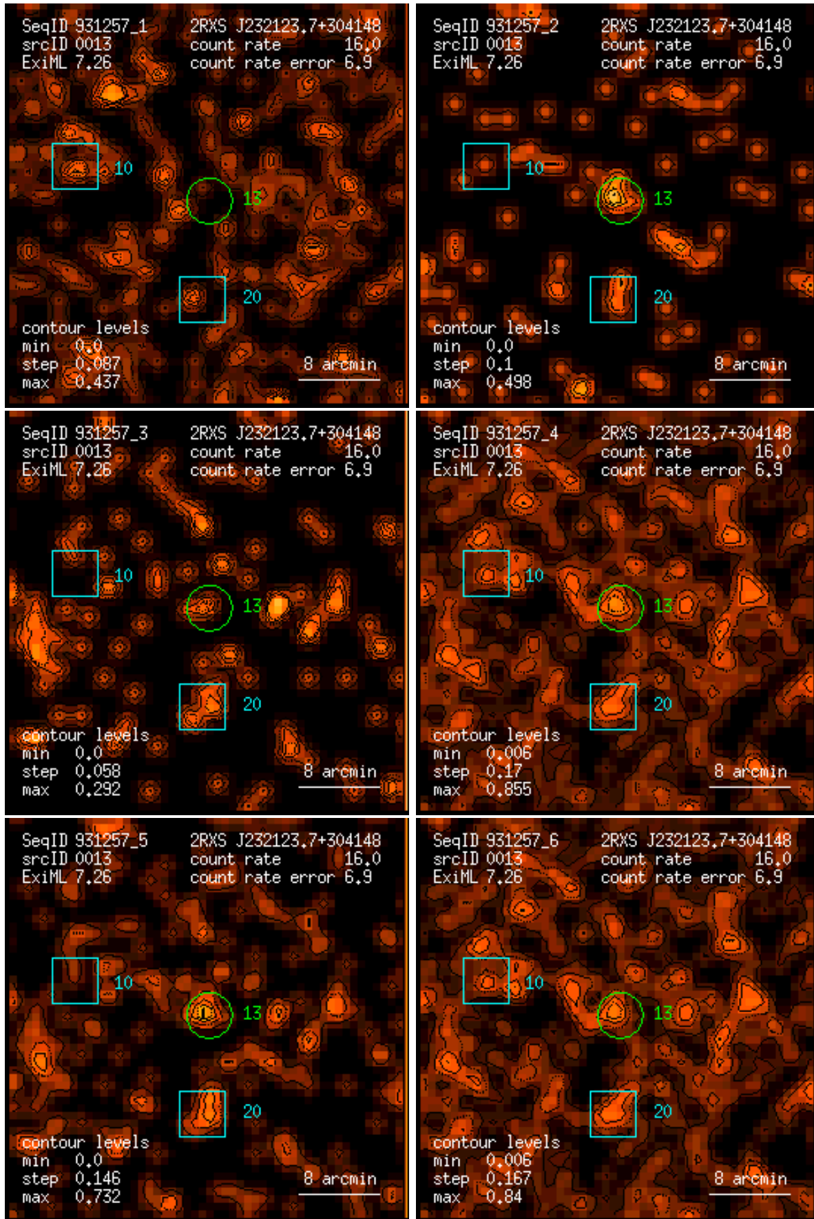
Figure 13: RASS 931257: detection 0013: band rate images, Gaussian filter: (1) PSPC channels 11 – 41, (2) 52 – 90, (3) 91 – 201, (4) 11 – 235, (5) 52 – 201, (6) 11 – 201. Broad band rates in counts/ks. Band rate contour levels in counts/ks/arcmin 2 .
