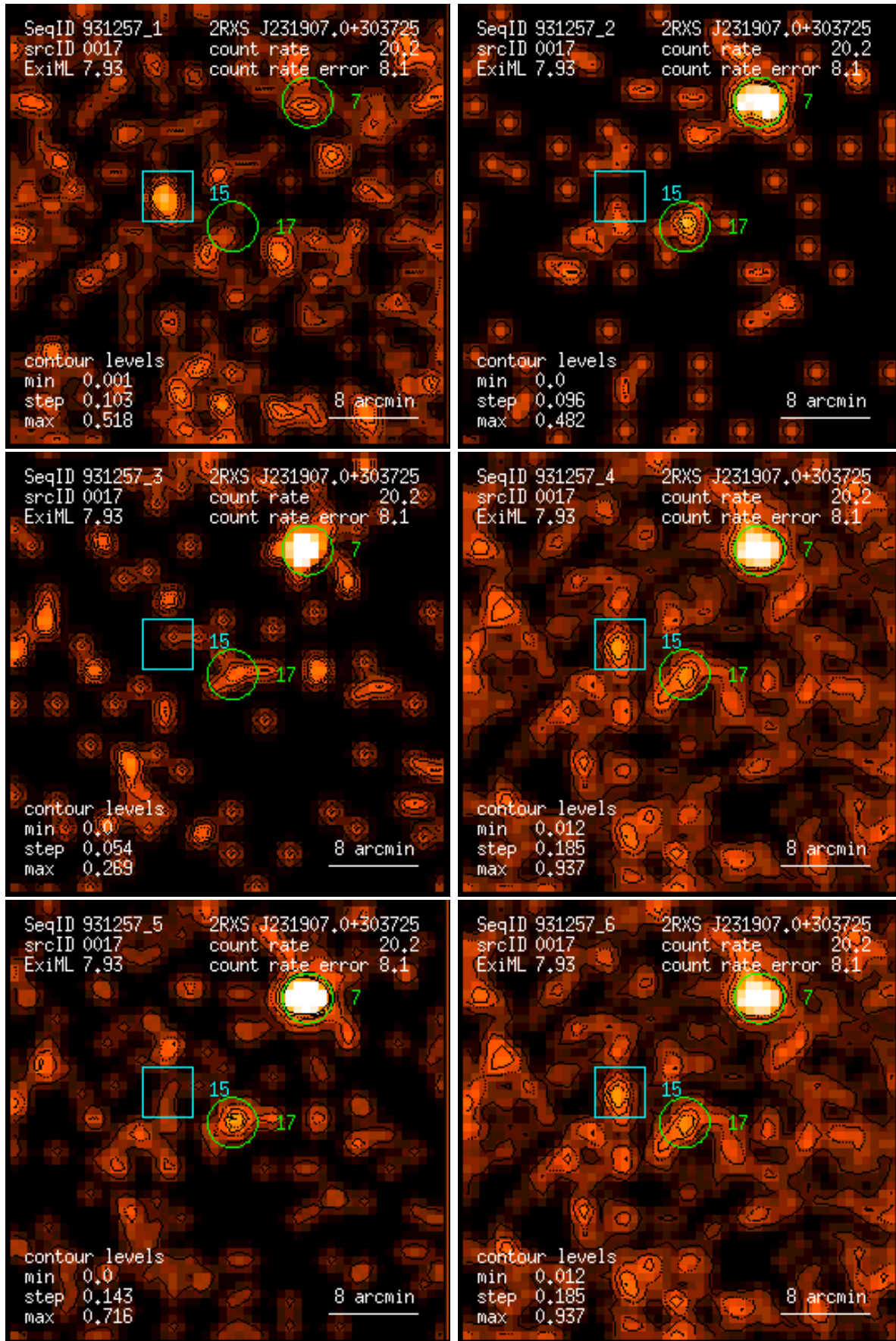
Figure 17: RASS 931257: detection 0017: band rate images, Gaussian filter: (1) PSPC channels 11 – 41, (2) 52 – 90, (3) 91 – 201, (4) 11 – 235, (5) 52 – 201, (6) 11 – 201. Broad band rates in counts/ks. Band rate contour levels in counts/ks/arcmin 2 .
