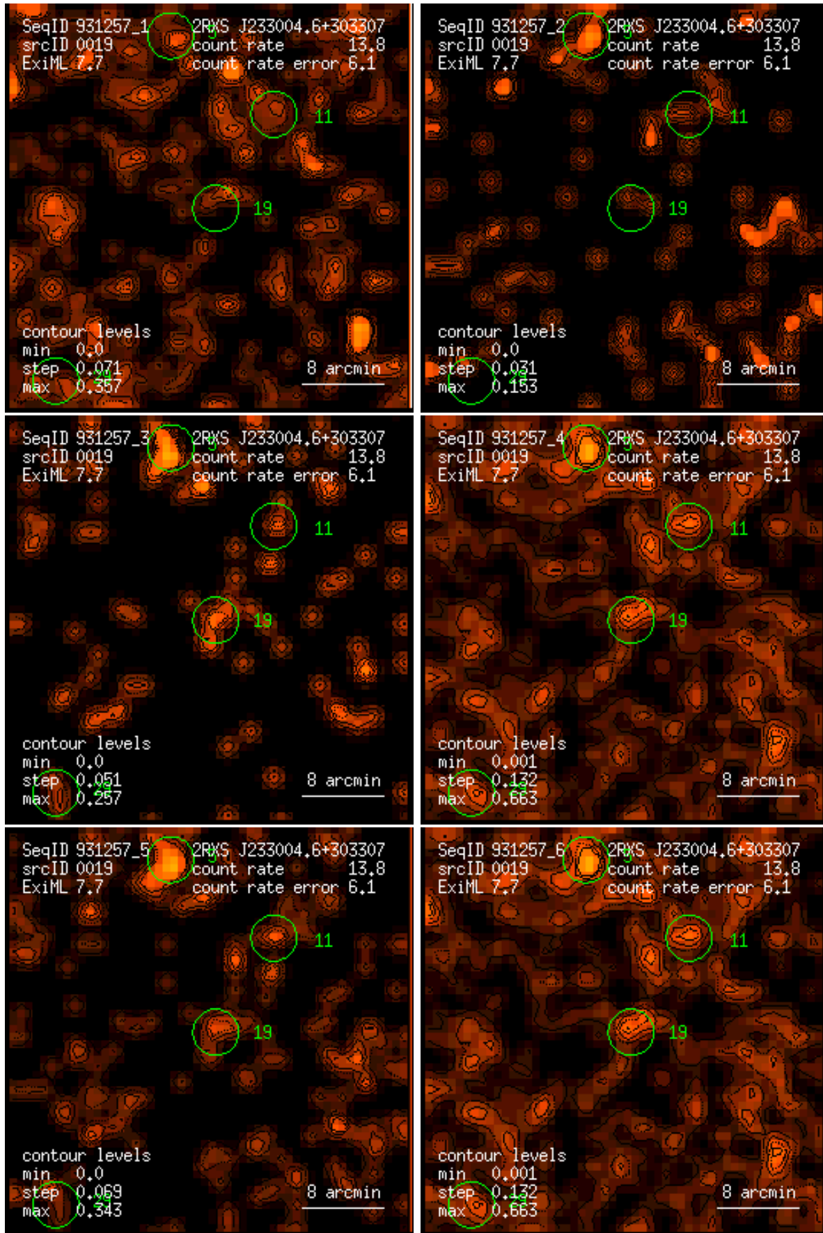
Figure 19: RASS 931257: detection 0019: band rate images, Gaussian filter: (1) PSPC channels 11 – 41, (2) 52 – 90, (3) 91 – 201, (4) 11 – 235, (5) 52 – 201, (6) 11 – 201. Broad band rates in counts/ks. Band rate contour levels in counts/ks/arcmin 2 .
