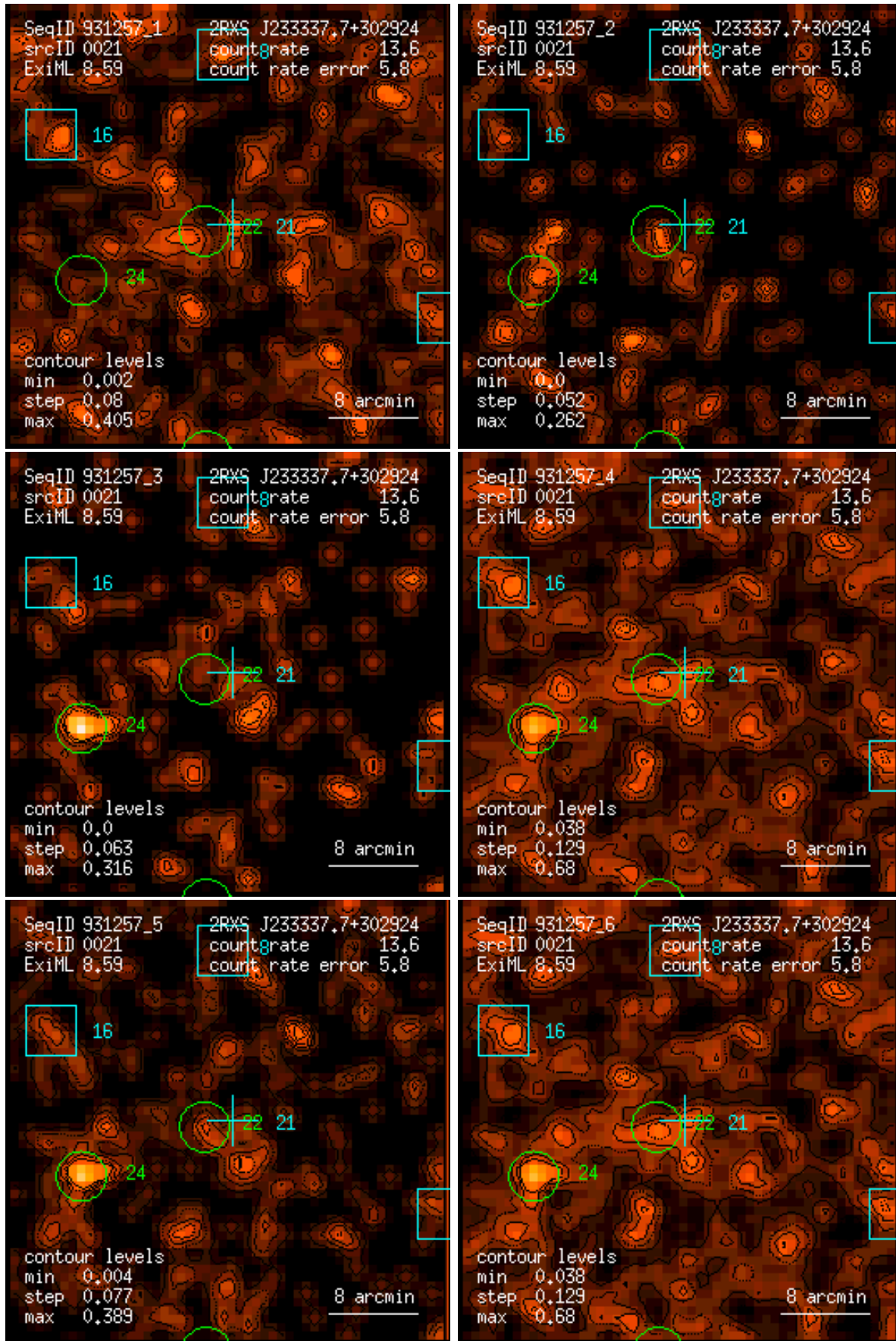
Figure 21: RASS 931257: detection 0021: band rate images, Gaussian filter: (1) PSPC channels 11 – 41, (2) 52 – 90, (3) 91 – 201, (4) 11 – 235, (5) 52 – 201, (6) 11 – 201. Broad band rates in counts/ks. Band rate contour levels in counts/ks/arcmin 2 .
