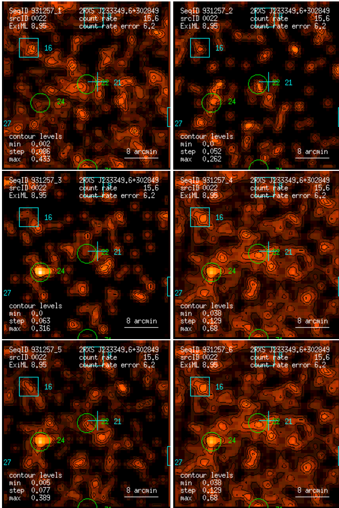
Figure 22: RASS 931257: detection 0022: band rate images, Gaussian filter: (1) PSPC channels 11 – 41, (2) 52 – 90, (3) 91 – 201, (4) 11 – 235, (5) 52 – 201, (6) 11 – 201. Broad band rates in counts/ks. Band rate contour levels in counts/ks/arcmin 2 .
