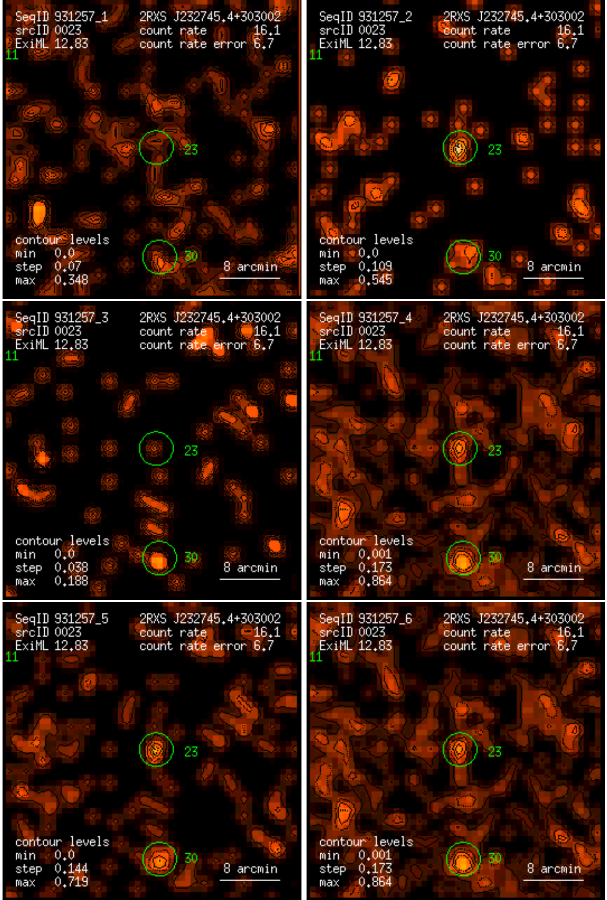
Figure 23: RASS 931257: detection 0023: band rate images, Gaussian filter: (1) PSPC channels 11 – 41, (2) 52 – 90, (3) 91 – 201, (4) 11 – 235, (5) 52 – 201, (6) 11 – 201. Broad band rates in counts/ks. Band rate contour levels in counts/ks/arcmin 2 .
