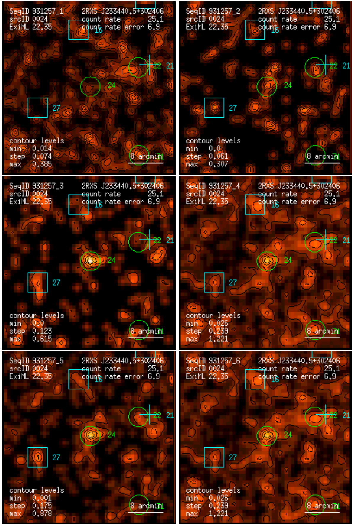
Figure 24: RASS 931257: detection 0024: band rate images, Gaussian filter: (1) PSPC channels 11 – 41, (2) 52 – 90, (3) 91 – 201, (4) 11 – 235, (5) 52 – 201, (6) 11 – 201. Broad band rates in counts/ks. Band rate contour levels in counts/ks/arcmin 2 .
