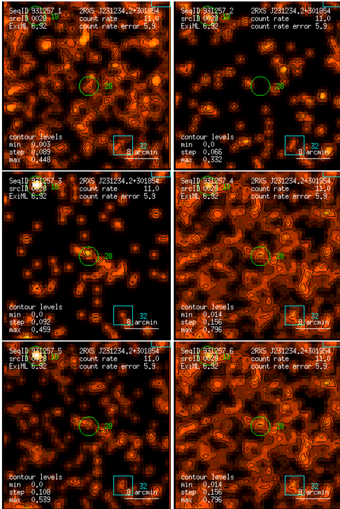
Figure 28: RASS 931257: detection 0028: band rate images, Gaussian filter: (1) PSPC channels 11 – 41, (2) 52 – 90, (3) 91 – 201, (4) 11 – 235, (5) 52 – 201, (6) 11 – 201. Broad band rates in counts/ks. Band rate contour levels in counts/ks/arcmin 2 .
