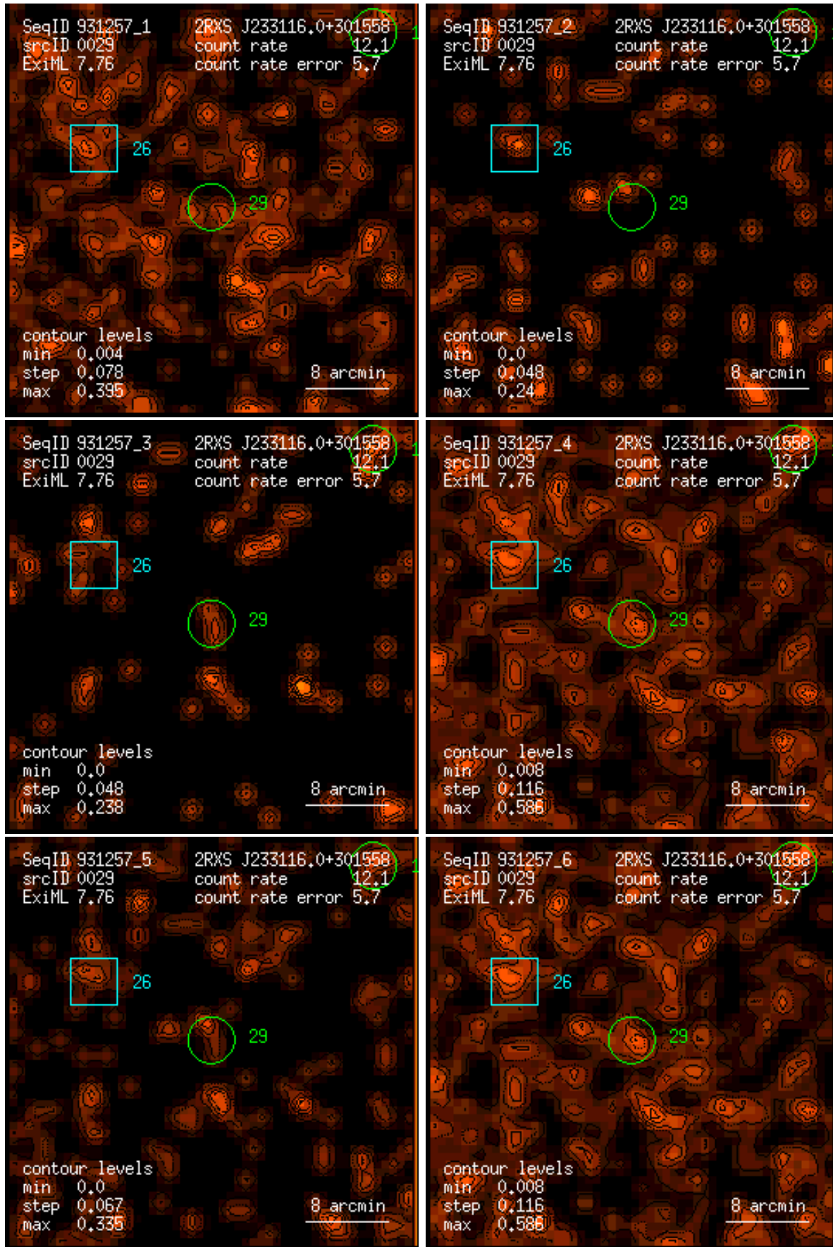
Figure 29: RASS 931257: detection 0029: band rate images, Gaussian filter: (1) PSPC channels 11 – 41, (2) 52 – 90, (3) 91 – 201, (4) 11 – 235, (5) 52 – 201, (6) 11 – 201. Broad band rates in counts/ks. Band rate contour levels in counts/ks/arcmin 2 .
