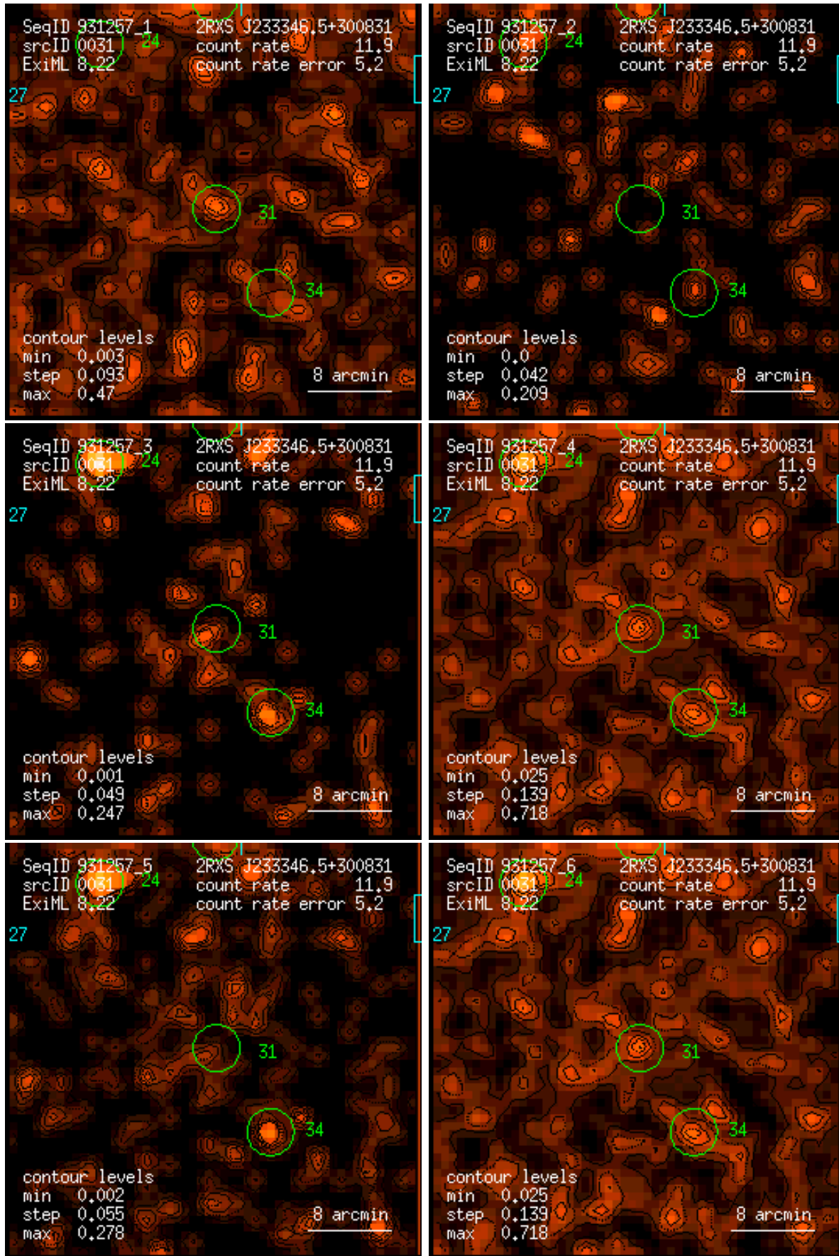
Figure 31: RASS 931257: detection 0031: band rate images, Gaussian filter: (1) PSPC channels 11 – 41, (2) 52 – 90, (3) 91 – 201, (4) 11 – 235, (5) 52 – 201, (6) 11 – 201. Broad band rates in counts/ks. Band rate contour levels in counts/ks/arcmin 2 .
