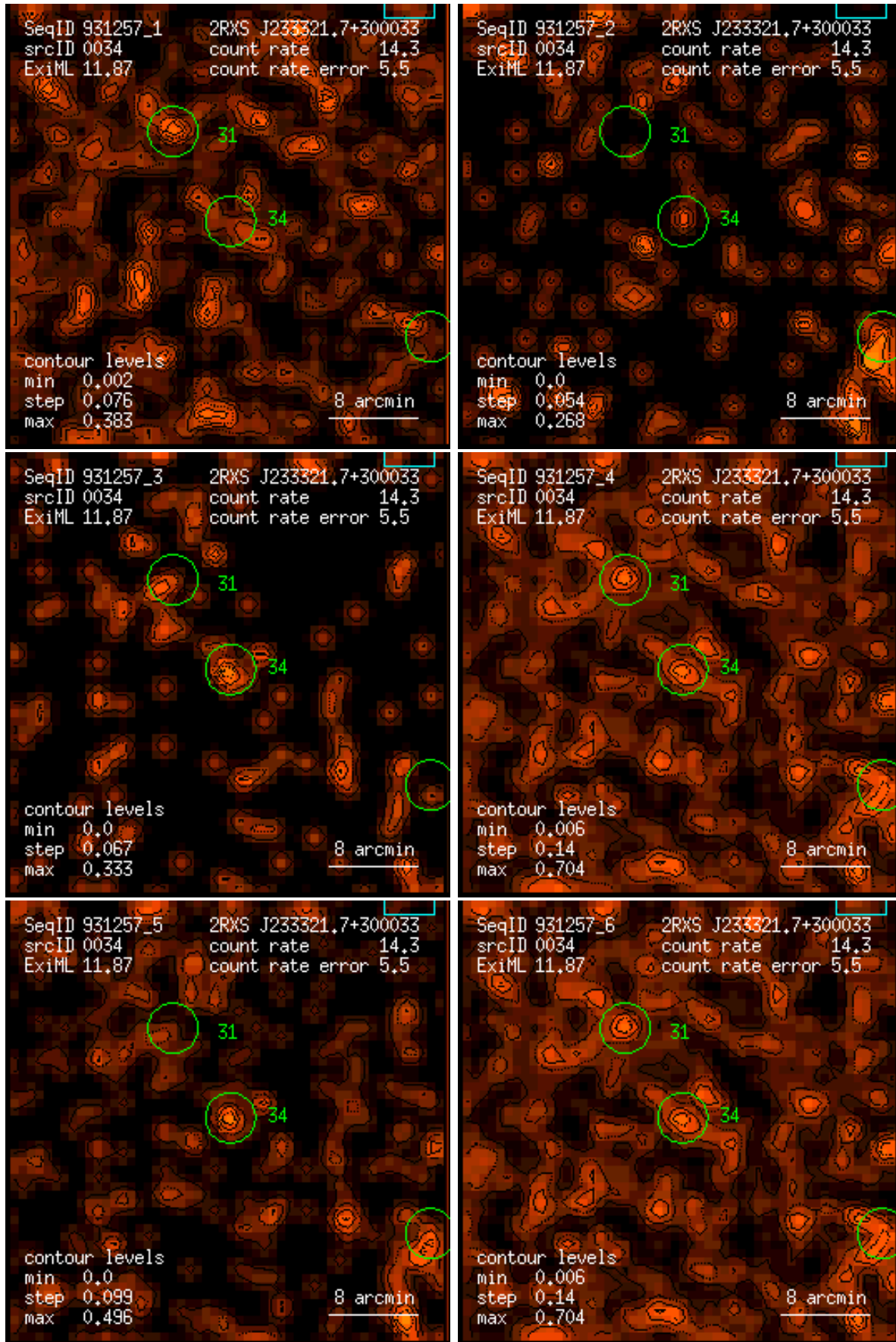
Figure 34: RASS 931257: detection 0034: band rate images, Gaussian filter: (1) PSPC channels 11 – 41, (2) 52 – 90, (3) 91 – 201, (4) 11 – 235, (5) 52 – 201, (6) 11 – 201. Broad band rates in counts/ks. Band rate contour levels in counts/ks/arcmin 2 .
