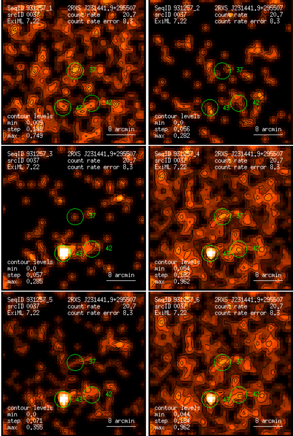
Figure 37: RASS 931257: detection 0037: band rate images, Gaussian filter: (1) PSPC channels 11 – 41, (2) 52 – 90, (3) 91 – 201, (4) 11 – 235, (5) 52 – 201, (6) 11 – 201. Broad band rates in counts/ks. Band rate contour levels in counts/ks/arcmin 2 .
