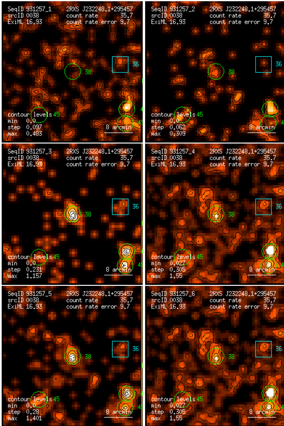
Figure 38: RASS 931257: detection 0038: band rate images, Gaussian filter: (1) PSPC channels 11 – 41, (2) 52 – 90, (3) 91 – 201, (4) 11 – 235, (5) 52 – 201, (6) 11 – 201. Broad band rates in counts/ks. Band rate contour levels in counts/ks/arcmin 2 .
