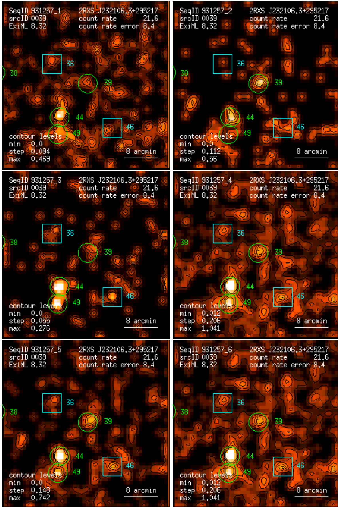
Figure 39: RASS 931257: detection 0039: band rate images, Gaussian filter: (1) PSPC channels 11 – 41, (2) 52 – 90, (3) 91 – 201, (4) 11 – 235, (5) 52 – 201, (6) 11 – 201. Broad band rates in counts/ks. Band rate contour levels in counts/ks/arcmin 2 .
