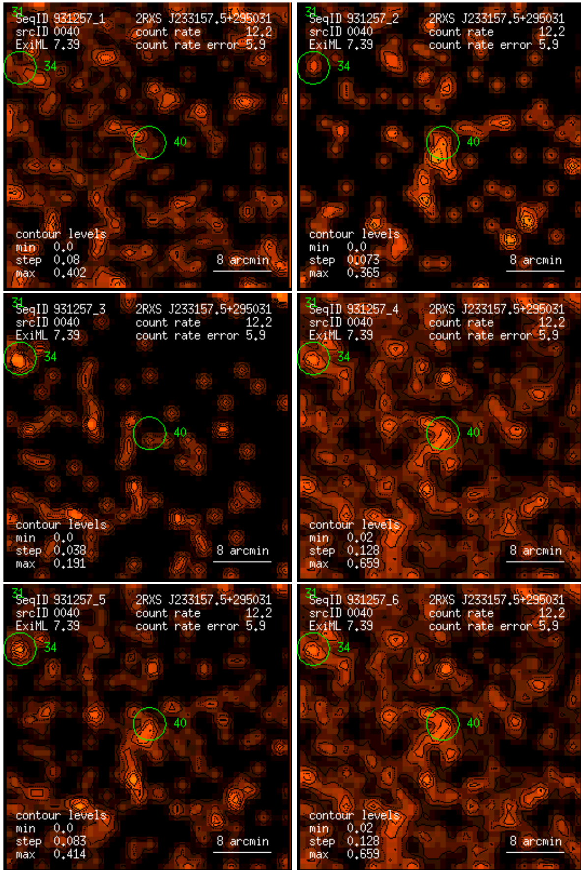
Figure 40: RASS 931257: detection 0040: band rate images, Gaussian filter: (1) PSPC channels 11 – 41, (2) 52 – 90, (3) 91 – 201, (4) 11 – 235, (5) 52 – 201, (6) 11 – 201. Broad band rates in counts/ks. Band rate contour levels in counts/ks/arcmin 2 .
