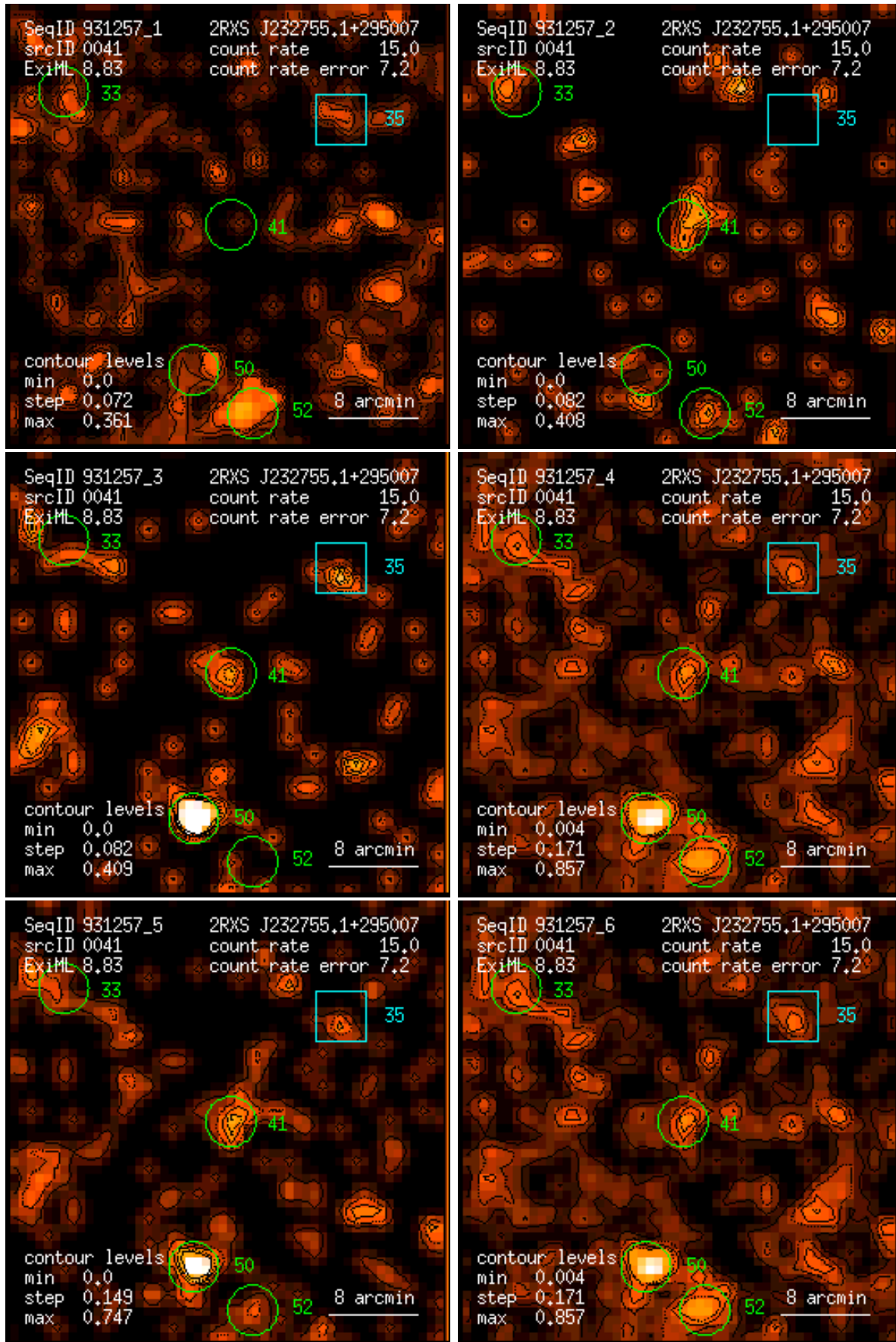
Figure 41: RASS 931257: detection 0041: band rate images, Gaussian filter: (1) PSPC channels 11 – 41, (2) 52 – 90, (3) 91 – 201, (4) 11 – 235, (5) 52 – 201, (6) 11 – 201. Broad band rates in counts/ks. Band rate contour levels in counts/ks/arcmin 2 .
