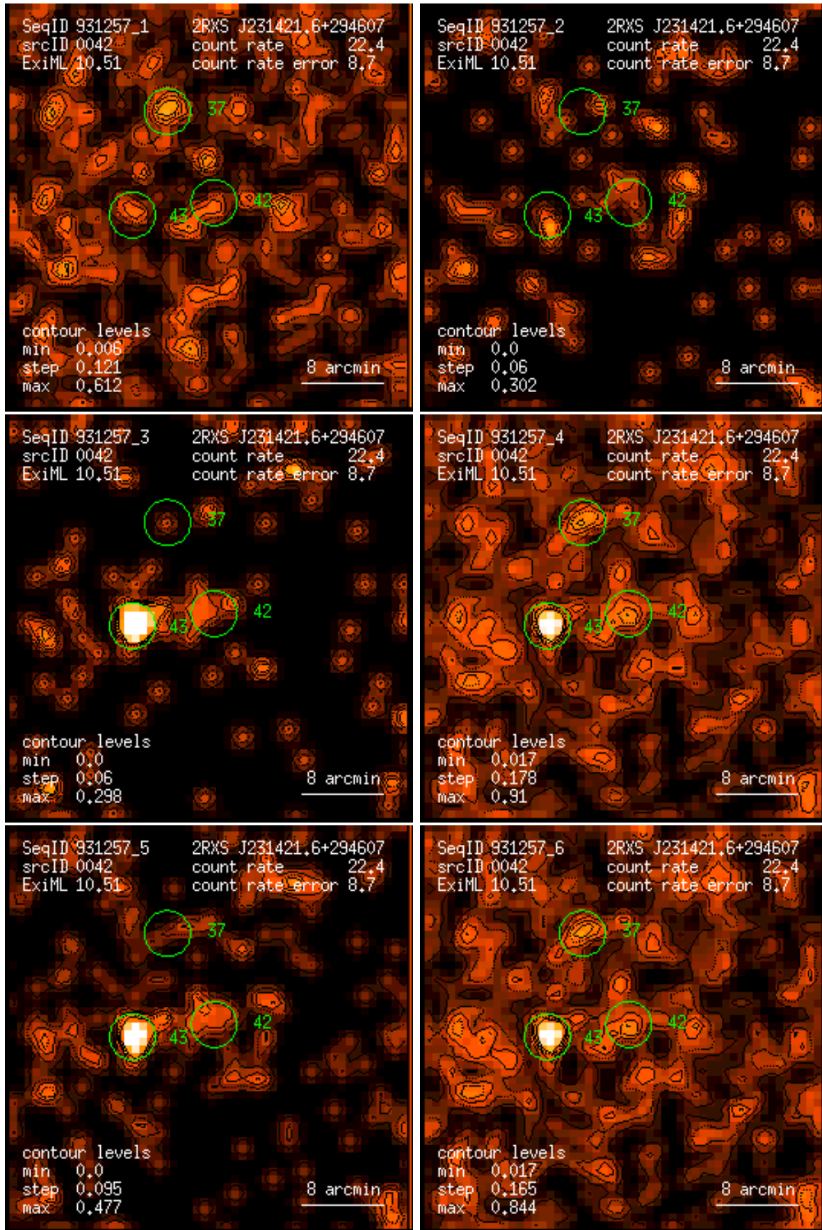
Figure 42: RASS 931257: detection 0042: band rate images, Gaussian filter: (1) PSPC channels 11 – 41, (2) 52 – 90, (3) 91 – 201, (4) 11 – 235, (5) 52 – 201, (6) 11 – 201. Broad band rates in counts/ks. Band rate contour levels in counts/ks/arcmin 2 .
