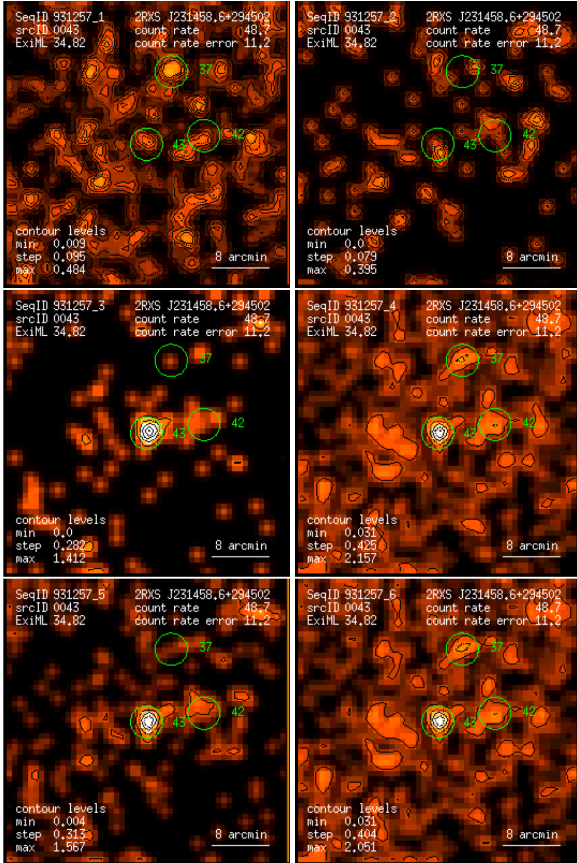
Figure 43: RASS 931257: detection 0043: band rate images, Gaussian filter: (1) PSPC channels 11 – 41, (2) 52 – 90, (3) 91 – 201, (4) 11 – 235, (5) 52 – 201, (6) 11 – 201. Broad band rates in counts/ks. Band rate contour levels in counts/ks/arcmin 2 .
