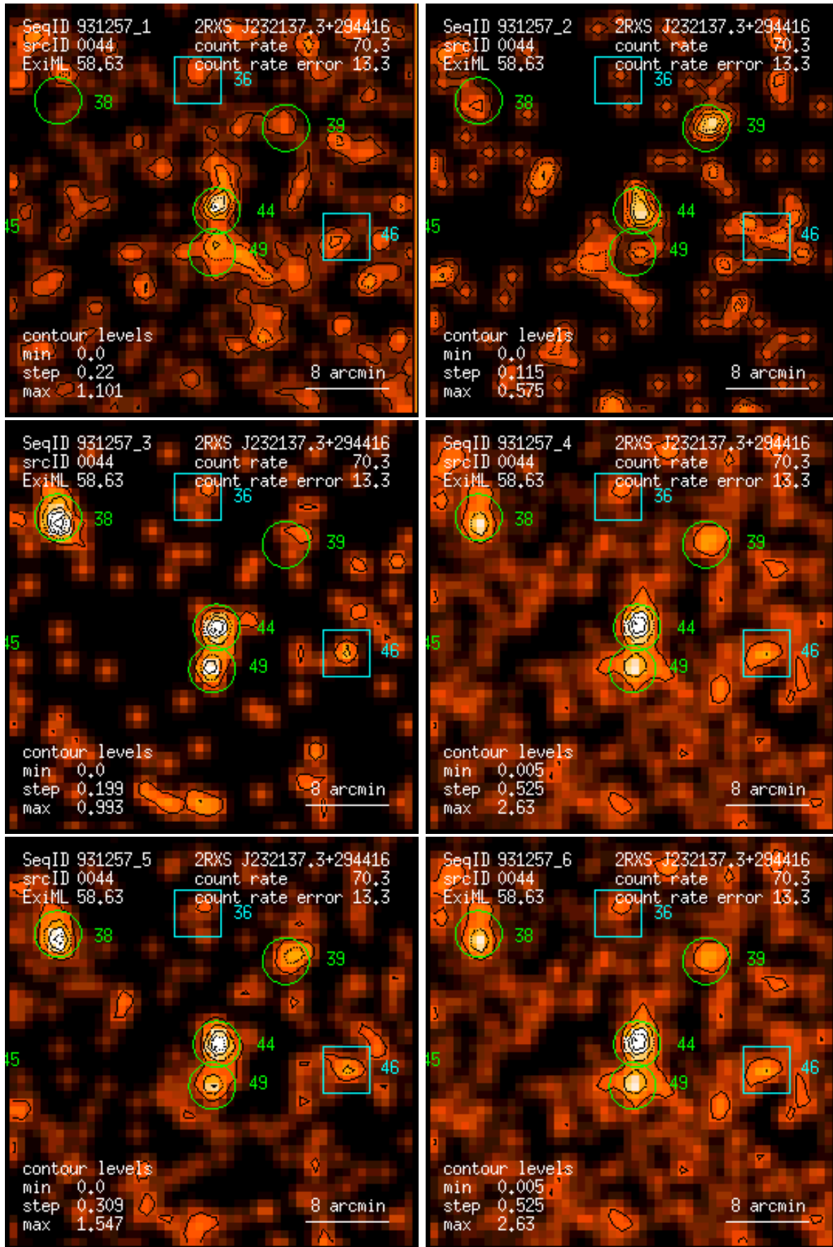
Figure 44: RASS 931257: detection 0044: band rate images, Gaussian filter: (1) PSPC channels 11 – 41, (2) 52 – 90, (3) 91 – 201, (4) 11 – 235, (5) 52 – 201, (6) 11 – 201. Broad band rates in counts/ks. Band rate contour levels in counts/ks/arcmin 2 .
