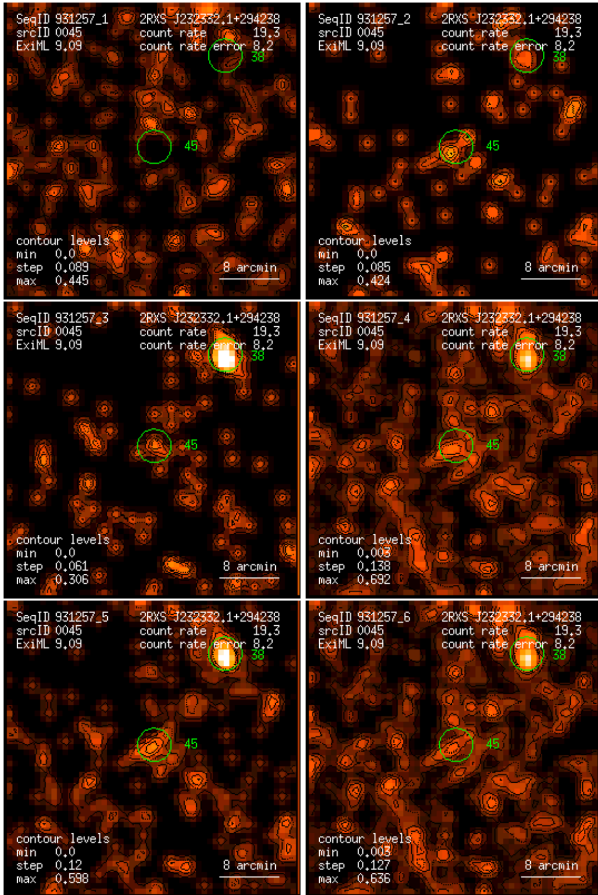
Figure 45: RASS 931257: detection 0045: band rate images, Gaussian filter: (1) PSPC channels 11 – 41, (2) 52 – 90, (3) 91 – 201, (4) 11 – 235, (5) 52 – 201, (6) 11 – 201. Broad band rates in counts/ks. Band rate contour levels in counts/ks/arcmin 2 .
