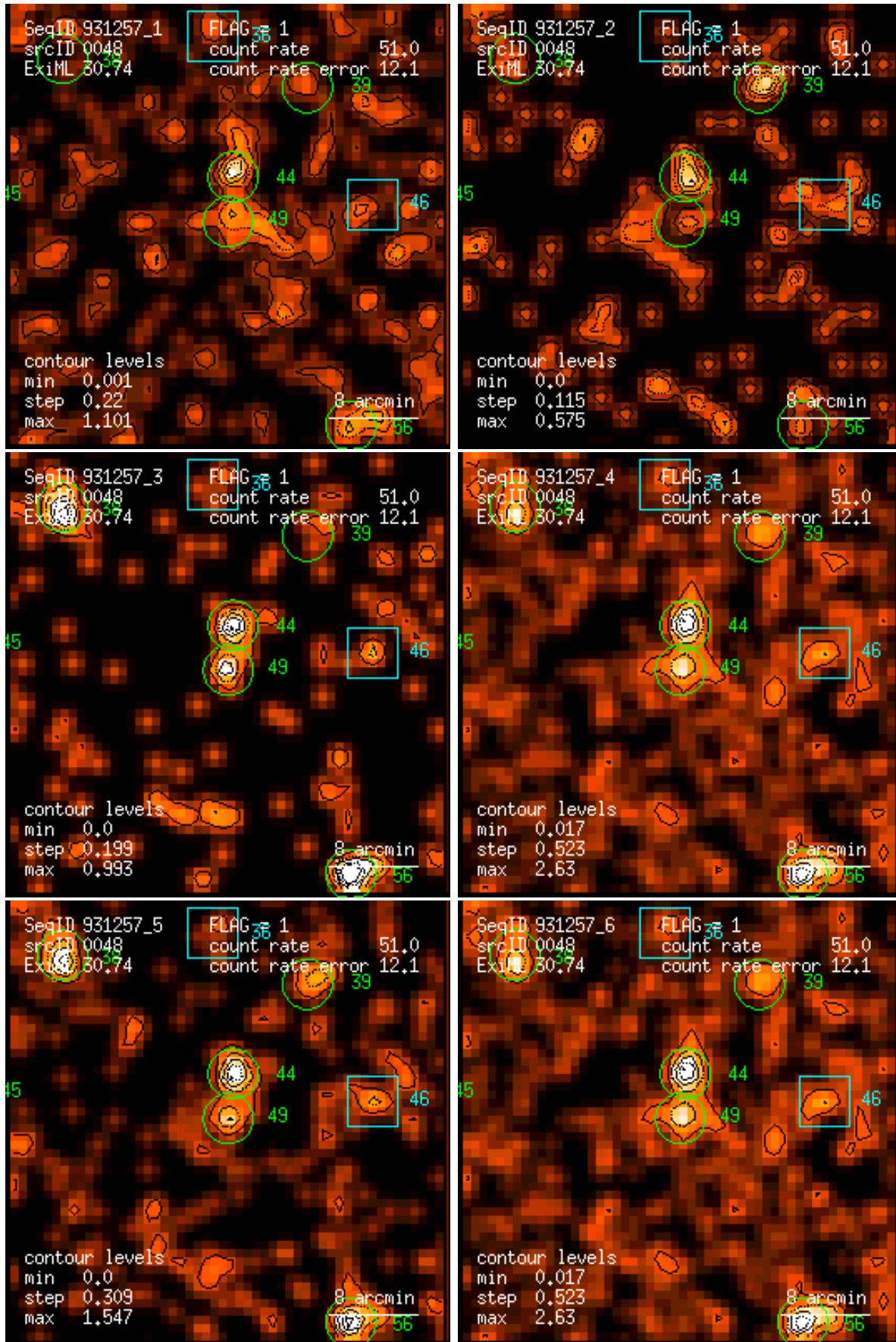
Figure 48: RASS 931257: detection 0048: band rate images, Gaussian filter: (1) PSPC channels 11 – 41, (2) 52 – 90, (3) 91 – 201, (4) 11 – 235, (5) 52 – 201, (6) 11 – 201. Broad band rates in counts/ks. Band rate contour levels in counts/ks/arcmin 2 .
