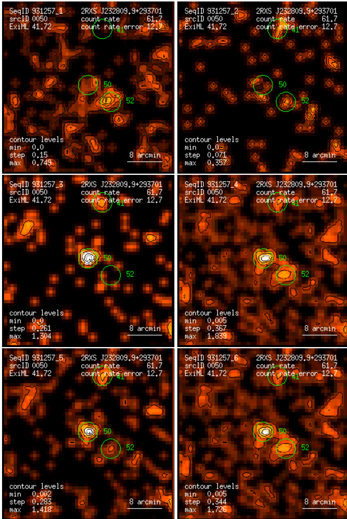
Figure 50: RASS 931257: detection 0050: band rate images, Gaussian filter: (1) PSPC channels 11 – 41, (2) 52 – 90, (3) 91 – 201, (4) 11 – 235, (5) 52 – 201, (6) 11 – 201. Broad band rates in counts/ks. Band rate contour levels in counts/ks/arcmin 2 .
