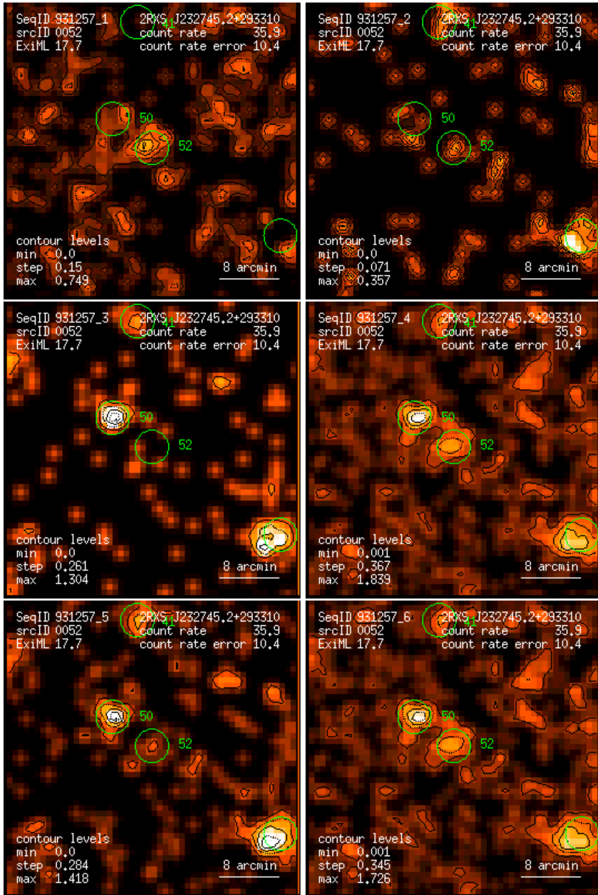
Figure 52: RASS 931257: detection 0052: band rate images, Gaussian filter: (1) PSPC channels 11 – 41, (2) 52 – 90, (3) 91 – 201, (4) 11 – 235, (5) 52 – 201, (6) 11 – 201. Broad band rates in counts/ks. Band rate contour levels in counts/ks/arcmin 2 .
