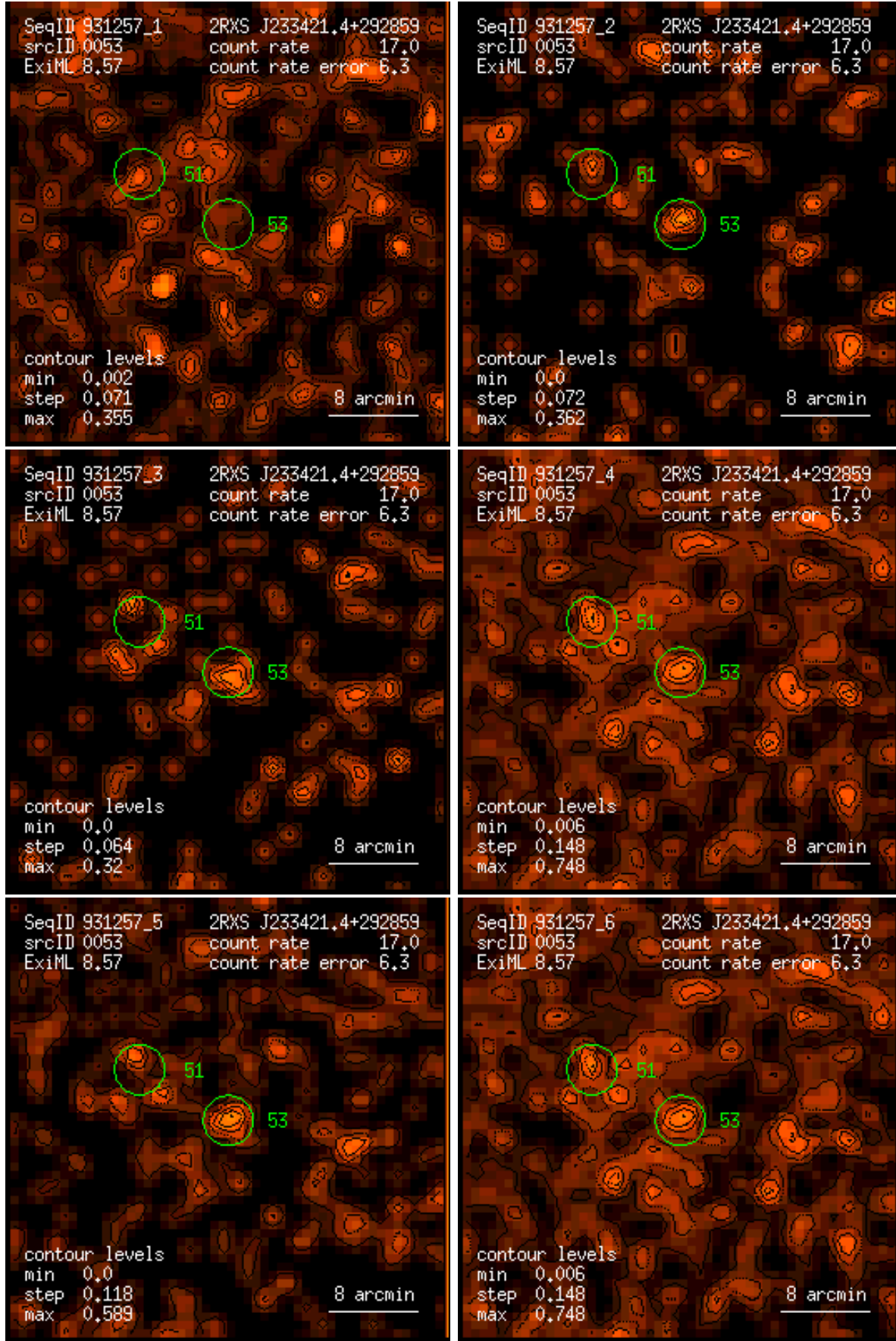
Figure 53: RASS 931257: detection 0053: band rate images, Gaussian filter: (1) PSPC channels 11 – 41, (2) 52 – 90, (3) 91 – 201, (4) 11 – 235, (5) 52 – 201, (6) 11 – 201. Broad band rates in counts/ks. Band rate contour levels in counts/ks/arcmin 2 .
