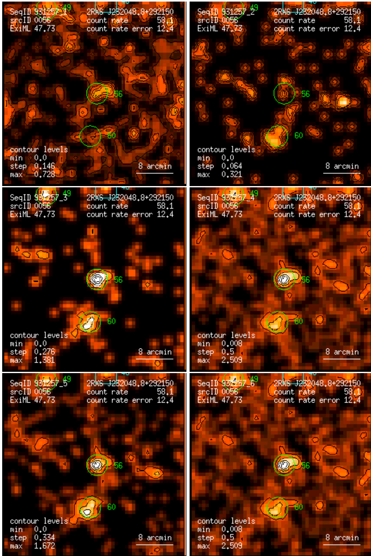
Figure 56: RASS 931257: detection 0056: band rate images, Gaussian filter: (1) PSPC channels 11 – 41, (2) 52 – 90, (3) 91 – 201, (4) 11 – 235, (5) 52 – 201, (6) 11 – 201. Broad band rates in counts/ks. Band rate contour levels in counts/ks/arcmin 2 .
