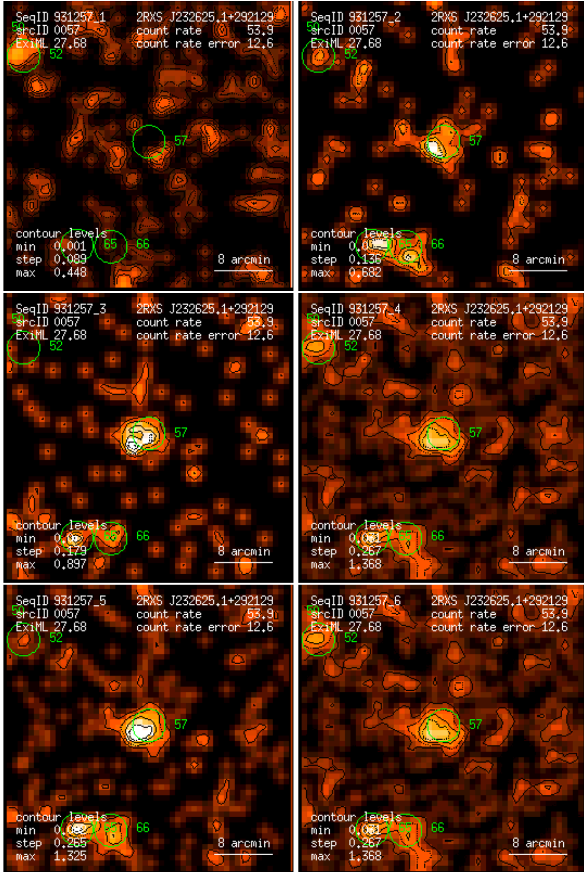
Figure 57: RASS 931257: detection 0057: band rate images, Gaussian filter: (1) PSPC channels 11 – 41, (2) 52 – 90, (3) 91 – 201, (4) 11 – 235, (5) 52 – 201, (6) 11 – 201. Broad band rates in counts/ks. Band rate contour levels in counts/ks/arcmin 2 .
