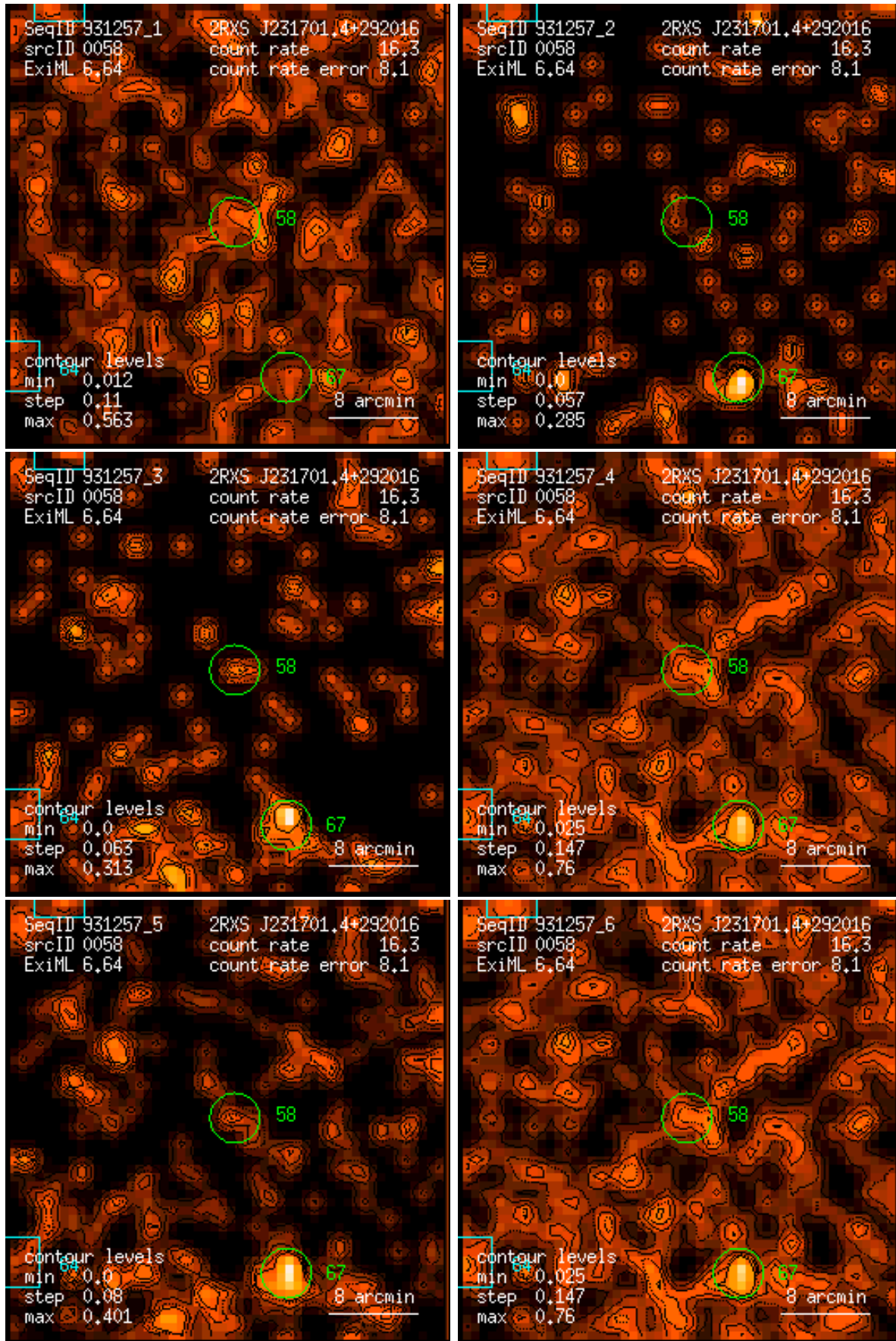
Figure 58: RASS 931257: detection 0058: band rate images, Gaussian filter: (1) PSPC channels 11 – 41, (2) 52 – 90, (3) 91 – 201, (4) 11 – 235, (5) 52 – 201, (6) 11 – 201. Broad band rates in counts/ks. Band rate contour levels in counts/ks/arcmin 2 .
