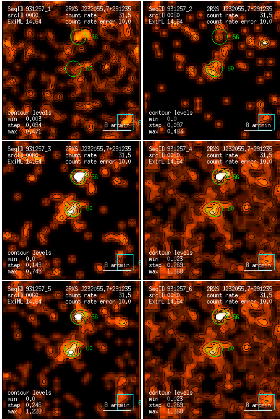
Figure 60: RASS 931257: detection 0060: band rate images, Gaussian filter: (1) PSPC channels 11 – 41, (2) 52 – 90, (3) 91 – 201, (4) 11 – 235, (5) 52 – 201, (6) 11 – 201. Broad band rates in counts/ks. Band rate contour levels in counts/ks/arcmin 2 .
