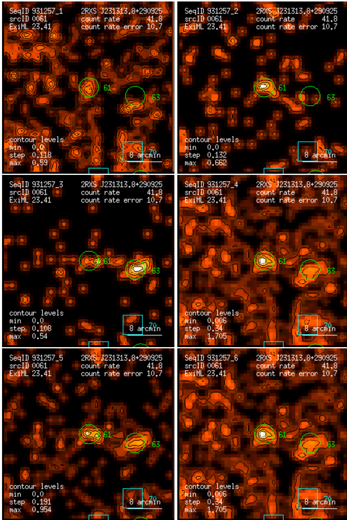
Figure 61: RASS 931257: detection 0061: band rate images, Gaussian filter: (1) PSPC channels 11 – 41, (2) 52 – 90, (3) 91 – 201, (4) 11 – 235, (5) 52 – 201, (6) 11 – 201. Broad band rates in counts/ks. Band rate contour levels in counts/ks/arcmin 2 .
