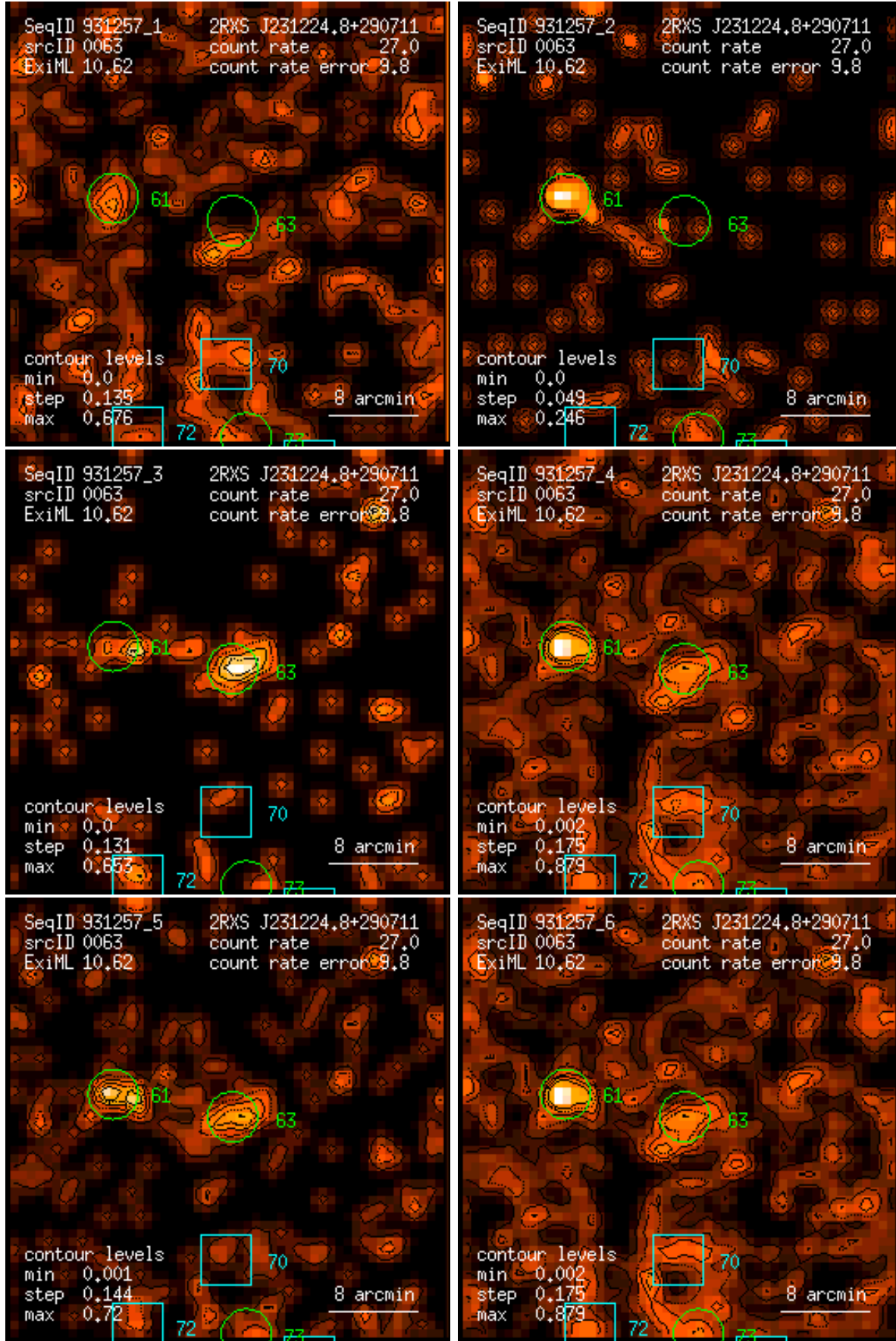
Figure 63: RASS 931257: detection 0063: band rate images, Gaussian filter: (1) PSPC channels 11 – 41, (2) 52 – 90, (3) 91 – 201, (4) 11 – 235, (5) 52 – 201, (6) 11 – 201. Broad band rates in counts/ks. Band rate contour levels in counts/ks/arcmin 2 .
