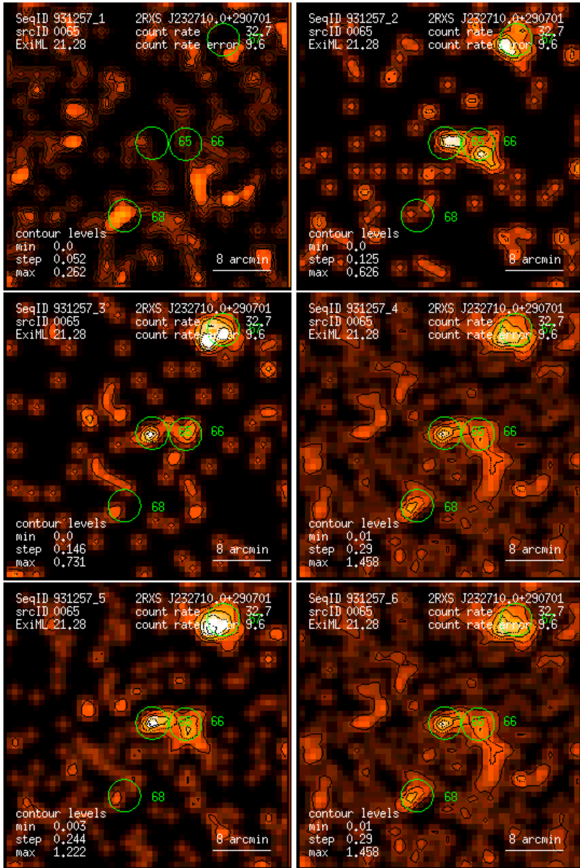
Figure 65: RASS 931257: detection 0065: band rate images, Gaussian filter: (1) PSPC channels 11 – 41, (2) 52 – 90, (3) 91 – 201, (4) 11 – 235, (5) 52 – 201, (6) 11 – 201. Broad band rates in counts/ks. Band rate contour levels in counts/ks/arcmin 2 .
