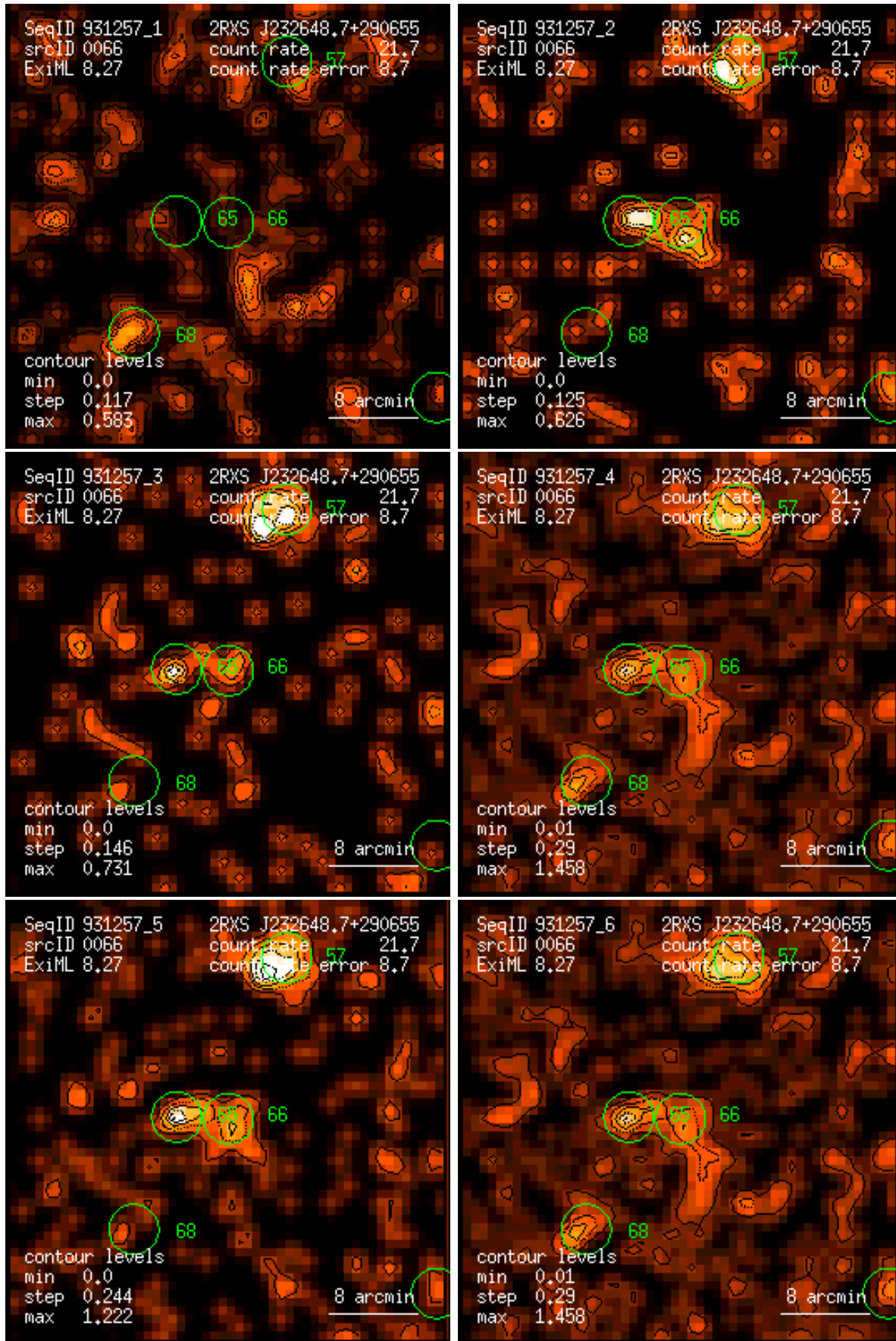
Figure 66: RASS 931257: detection 0066: band rate images, Gaussian filter: (1) PSPC channels 11 – 41, (2) 52 – 90, (3) 91 – 201, (4) 11 – 235, (5) 52 – 201, (6) 11 – 201. Broad band rates in counts/ks. Band rate contour levels in counts/ks/arcmin 2 .
