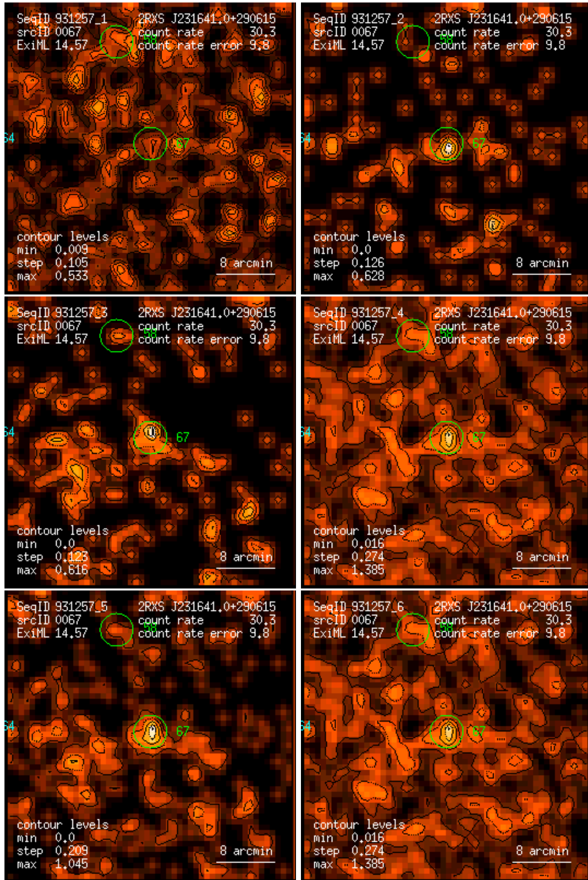
Figure 67: RASS 931257: detection 0067: band rate images, Gaussian filter: (1) PSPC channels 11 – 41, (2) 52 – 90, (3) 91 – 201, (4) 11 – 235, (5) 52 – 201, (6) 11 – 201. Broad band rates in counts/ks. Band rate contour levels in counts/ks/arcmin 2 .
