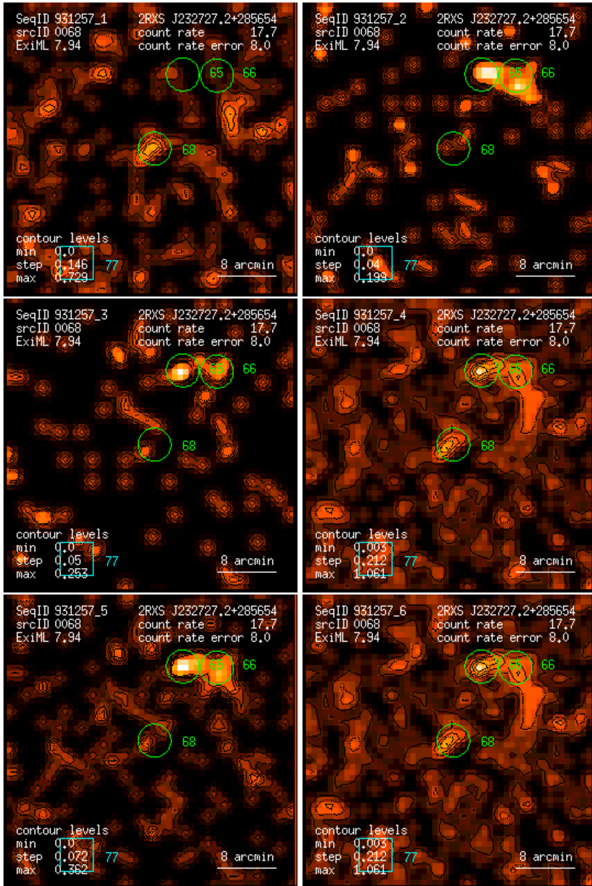
Figure 68: RASS 931257: detection 0068: band rate images, Gaussian filter: (1) PSPC channels 11 – 41, (2) 52 – 90, (3) 91 – 201, (4) 11 – 235, (5) 52 – 201, (6) 11 – 201. Broad band rates in counts/ks. Band rate contour levels in counts/ks/arcmin 2 .
