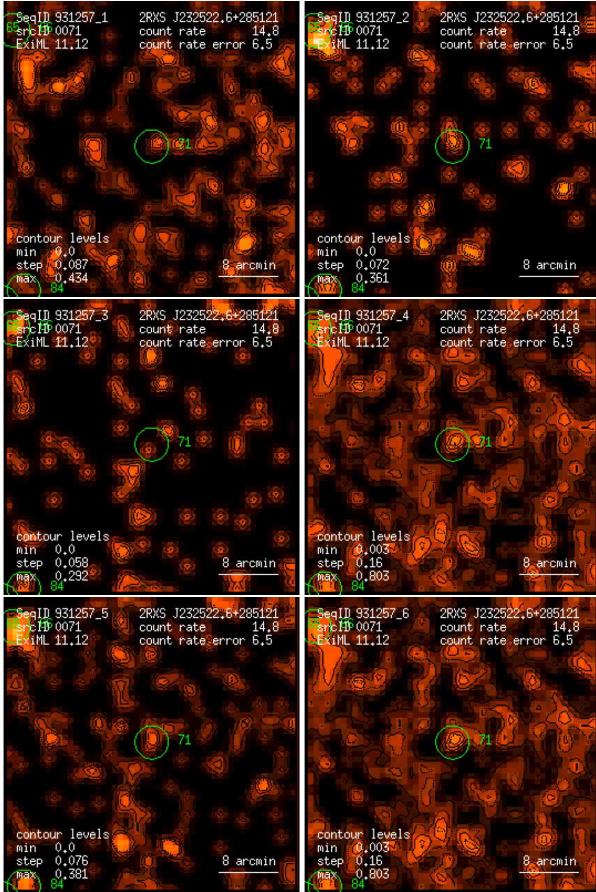
Figure 71: RASS 931257: detection 0071: band rate images, Gaussian filter: (1) PSPC channels 11 – 41, (2) 52 – 90, (3) 91 – 201, (4) 11 – 235, (5) 52 – 201, (6) 11 – 201. Broad band rates in counts/ks. Band rate contour levels in counts/ks/arcmin 2 .
