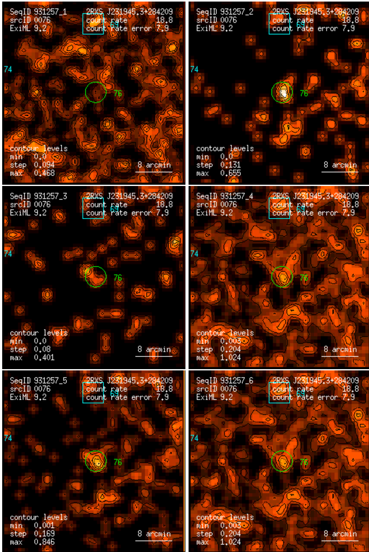
Figure 76: RASS 931257: detection 0076: band rate images, Gaussian filter: (1) PSPC channels 11 – 41, (2) 52 – 90, (3) 91 – 201, (4) 11 – 235, (5) 52 – 201, (6) 11 – 201. Broad band rates in counts/ks. Band rate contour levels in counts/ks/arcmin 2 .
