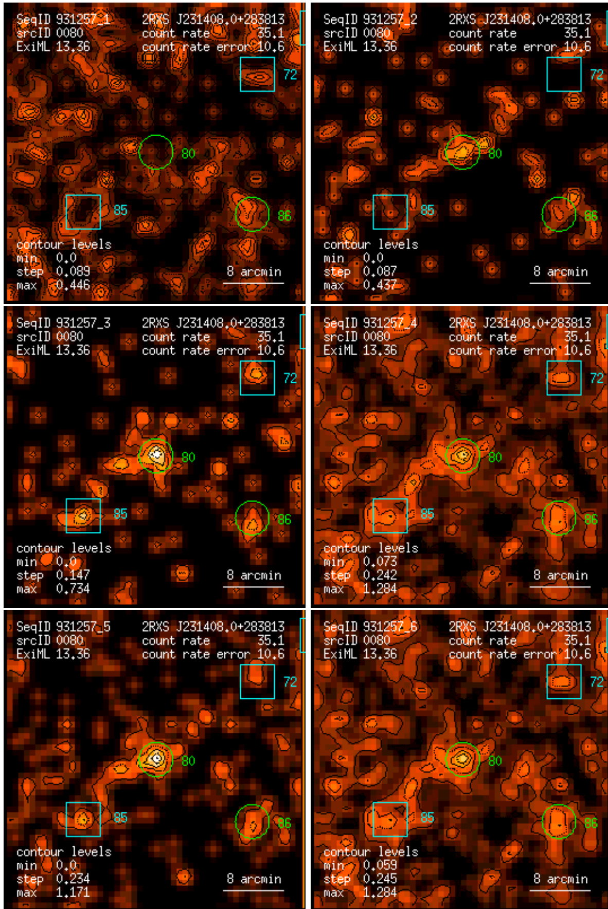
Figure 80: RASS 931257: detection 0080: band rate images, Gaussian filter: (1) PSPC channels 11 – 41, (2) 52 – 90, (3) 91 – 201, (4) 11 – 235, (5) 52 – 201, (6) 11 – 201. Broad band rates in counts/ks. Band rate contour levels in counts/ks/arcmin 2 .
