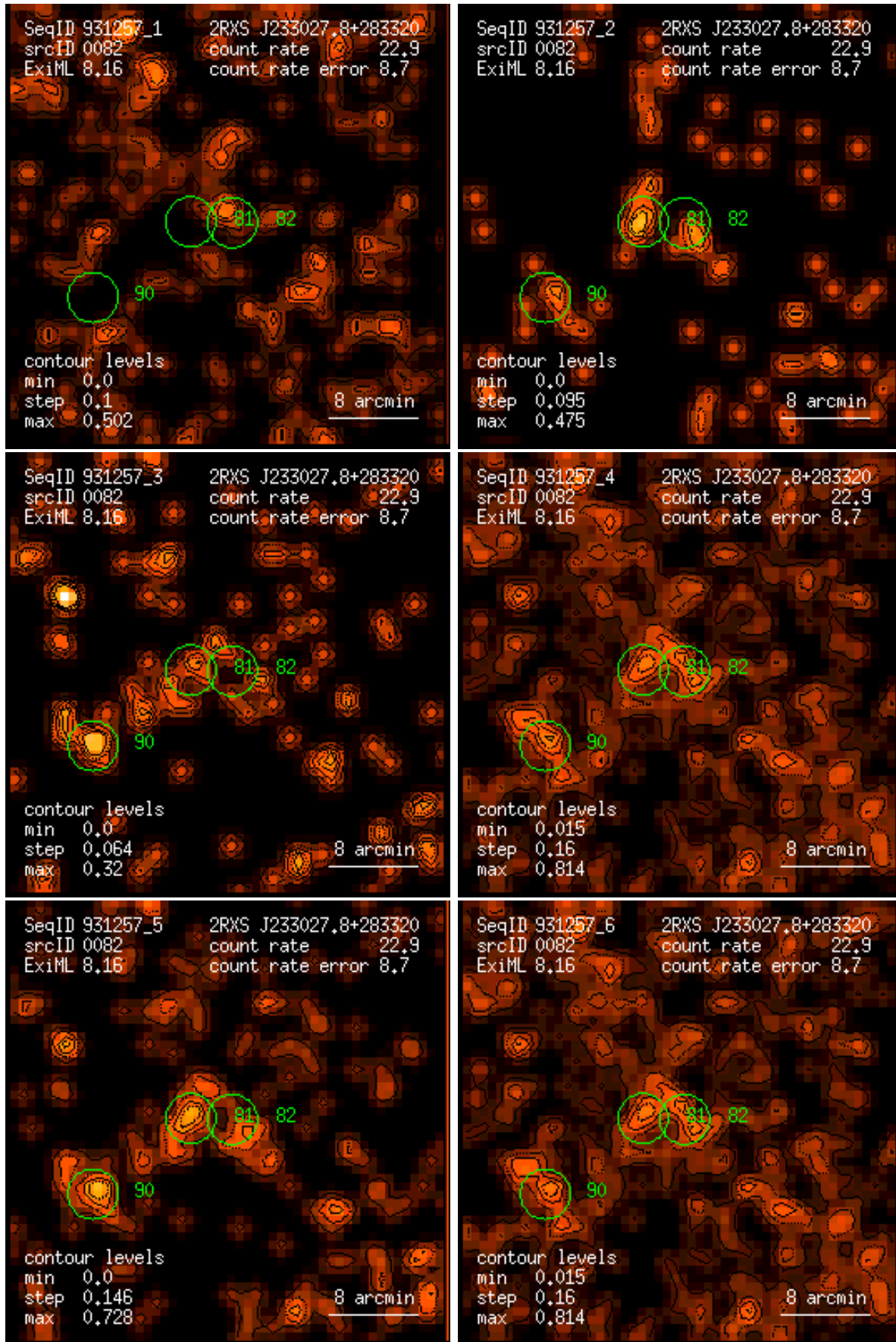
Figure 82: RASS 931257: detection 0082: band rate images, Gaussian filter: (1) PSPC channels 11 – 41, (2) 52 – 90, (3) 91 – 201, (4) 11 – 235, (5) 52 – 201, (6) 11 – 201. Broad band rates in counts/ks. Band rate contour levels in counts/ks/arcmin 2 .
