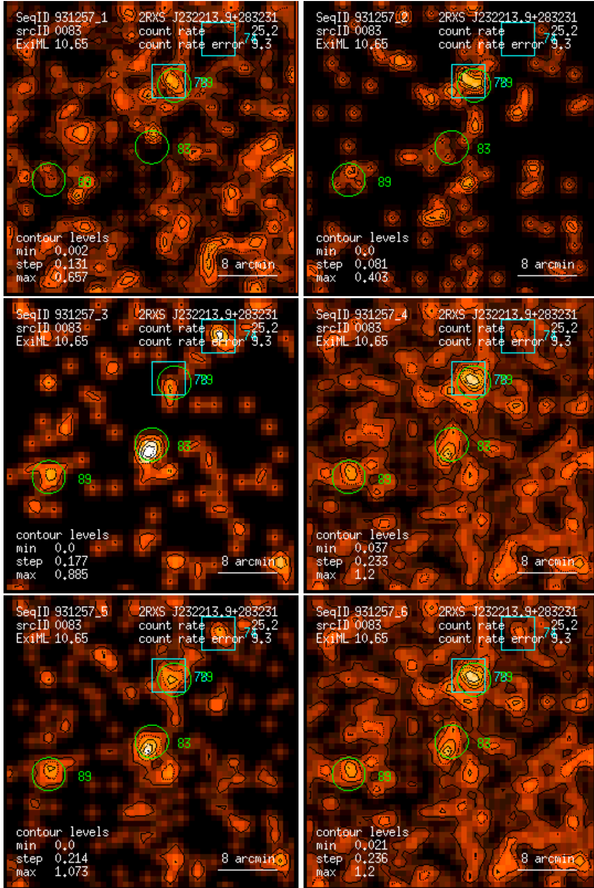
Figure 83: RASS 931257: detection 0083: band rate images, Gaussian filter: (1) PSPC channels 11 – 41, (2) 52 – 90, (3) 91 – 201, (4) 11 – 235, (5) 52 – 201, (6) 11 – 201. Broad band rates in counts/ks. Band rate contour levels in counts/ks/arcmin 2 .
