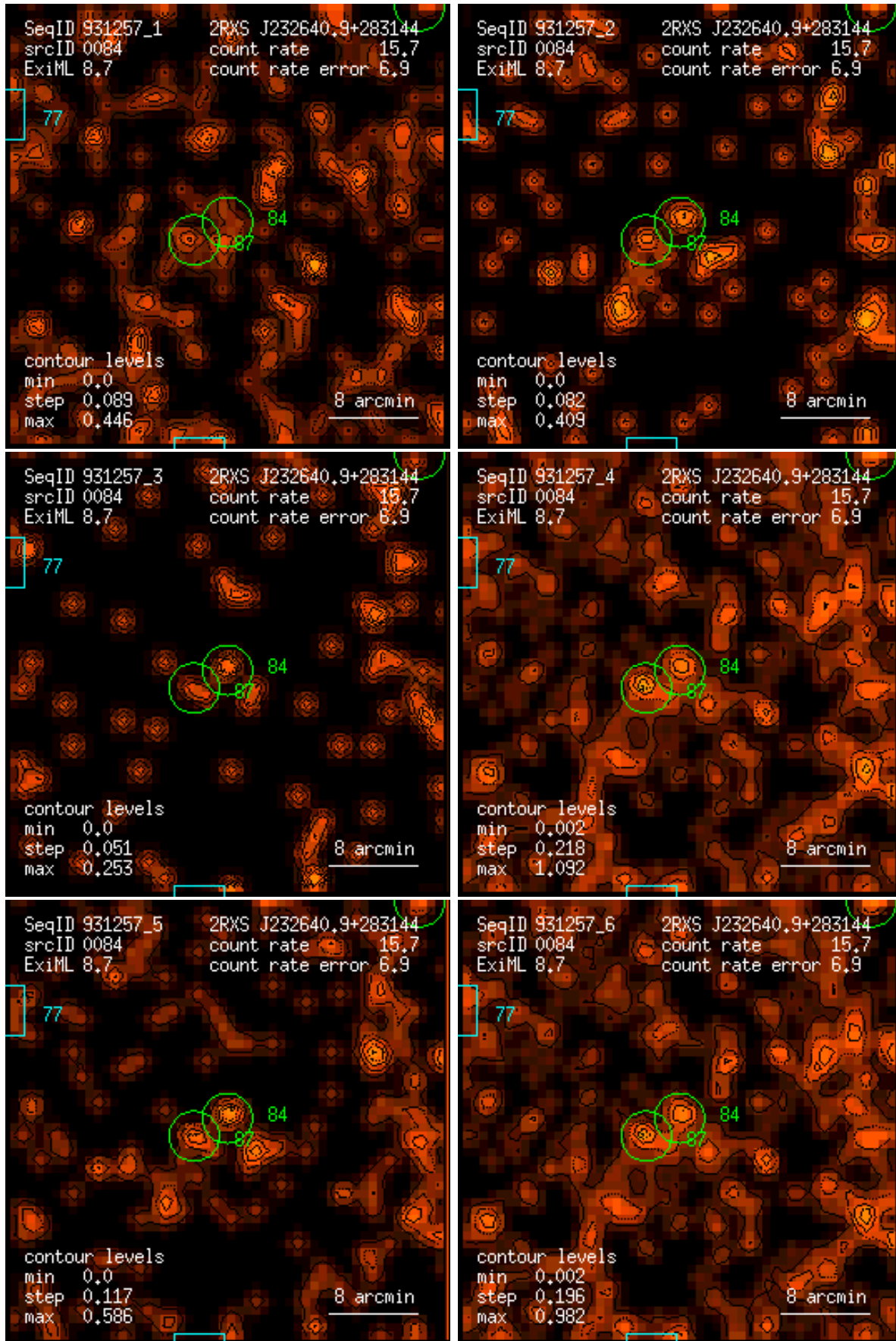
Figure 84: RASS 931257: detection 0084: band rate images, Gaussian filter: (1) PSPC channels 11 – 41, (2) 52 – 90, (3) 91 – 201, (4) 11 – 235, (5) 52 – 201, (6) 11 – 201. Broad band rates in counts/ks. Band rate contour levels in counts/ks/arcmin 2 .
