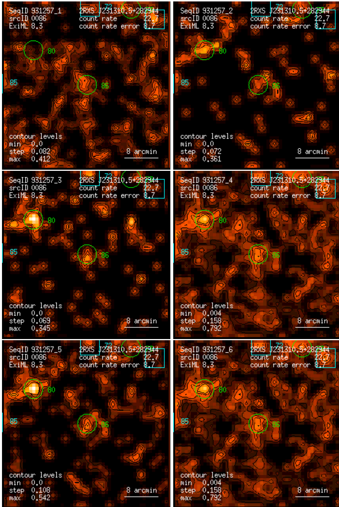
Figure 86: RASS 931257: detection 0086: band rate images, Gaussian filter: (1) PSPC channels 11 – 41, (2) 52 – 90, (3) 91 – 201, (4) 11 – 235, (5) 52 – 201, (6) 11 – 201. Broad band rates in counts/ks. Band rate contour levels in counts/ks/arcmin 2 .
