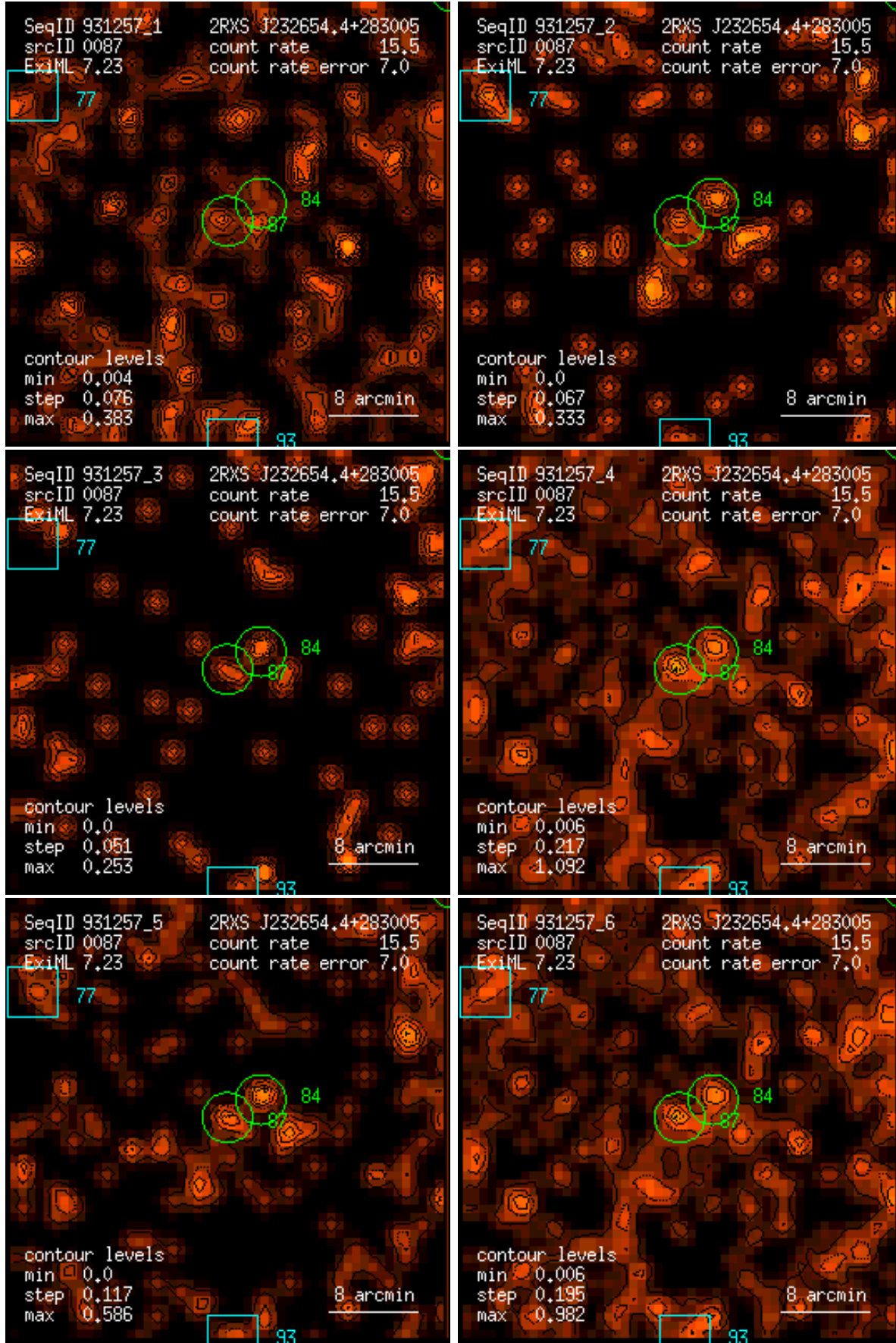
Figure 87: RASS 931257: detection 0087: band rate images, Gaussian filter: (1) PSPC channels 11 – 41, (2) 52 – 90, (3) 91 – 201, (4) 11 – 235, (5) 52 – 201, (6) 11 – 201. Broad band rates in counts/ks. Band rate contour levels in counts/ks/arcmin 2 .
