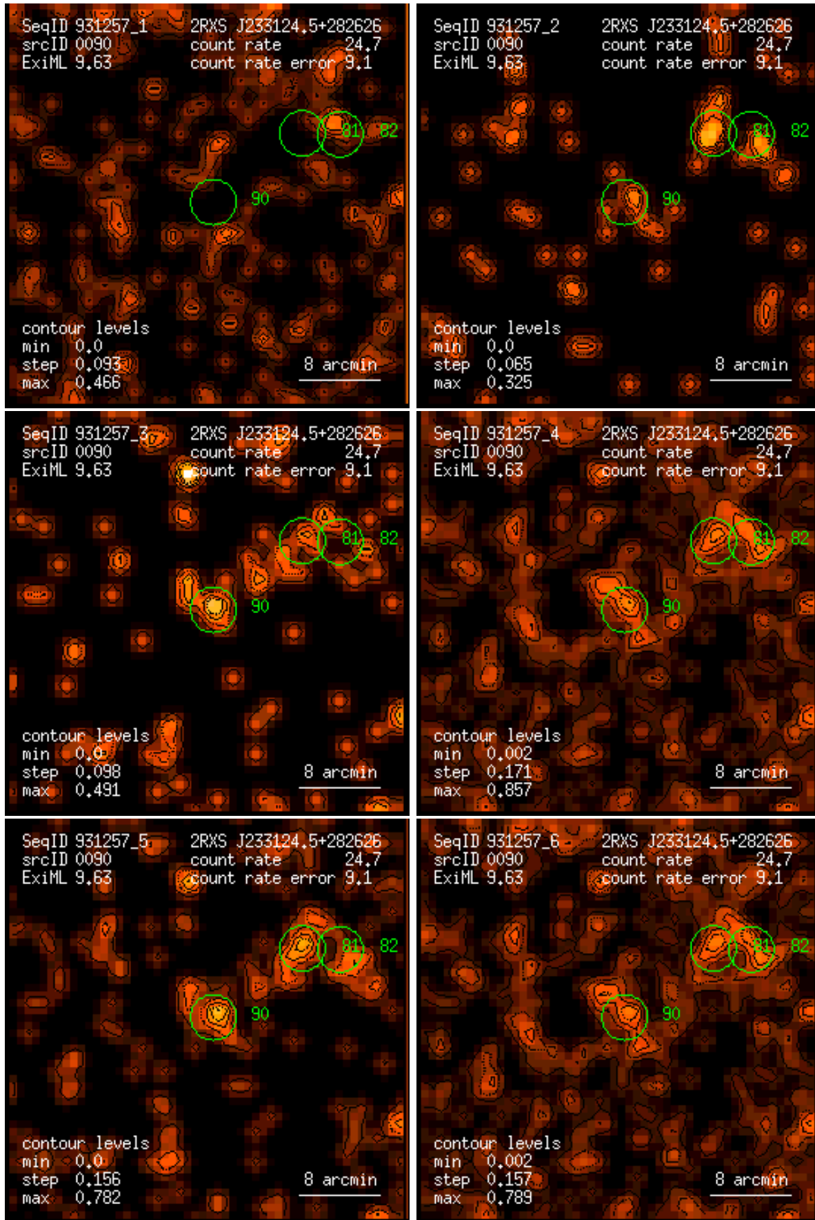
Figure 90: RASS 931257: detection 0090: band rate images, Gaussian filter: (1) PSPC channels 11 – 41, (2) 52 – 90, (3) 91 – 201, (4) 11 – 235, (5) 52 – 201, (6) 11 – 201. Broad band rates in counts/ks. Band rate contour levels in counts/ks/arcmin 2 .
