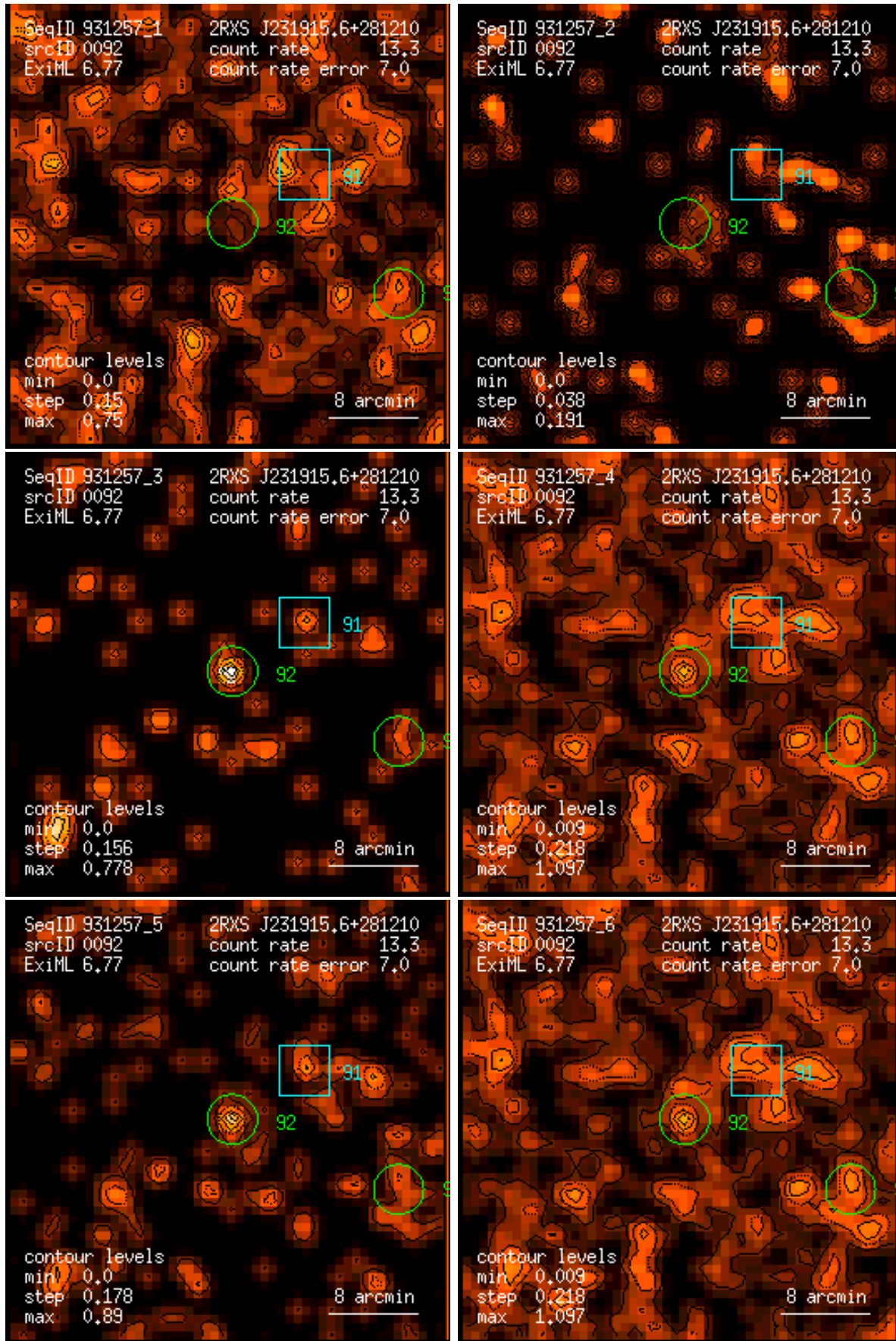
Figure 92: RASS 931257: detection 0092: band rate images, Gaussian filter: (1) PSPC channels 11 – 41, (2) 52 – 90, (3) 91 – 201, (4) 11 – 235, (5) 52 – 201, (6) 11 – 201. Broad band rates in counts/ks. Band rate contour levels in counts/ks/arcmin 2 .
