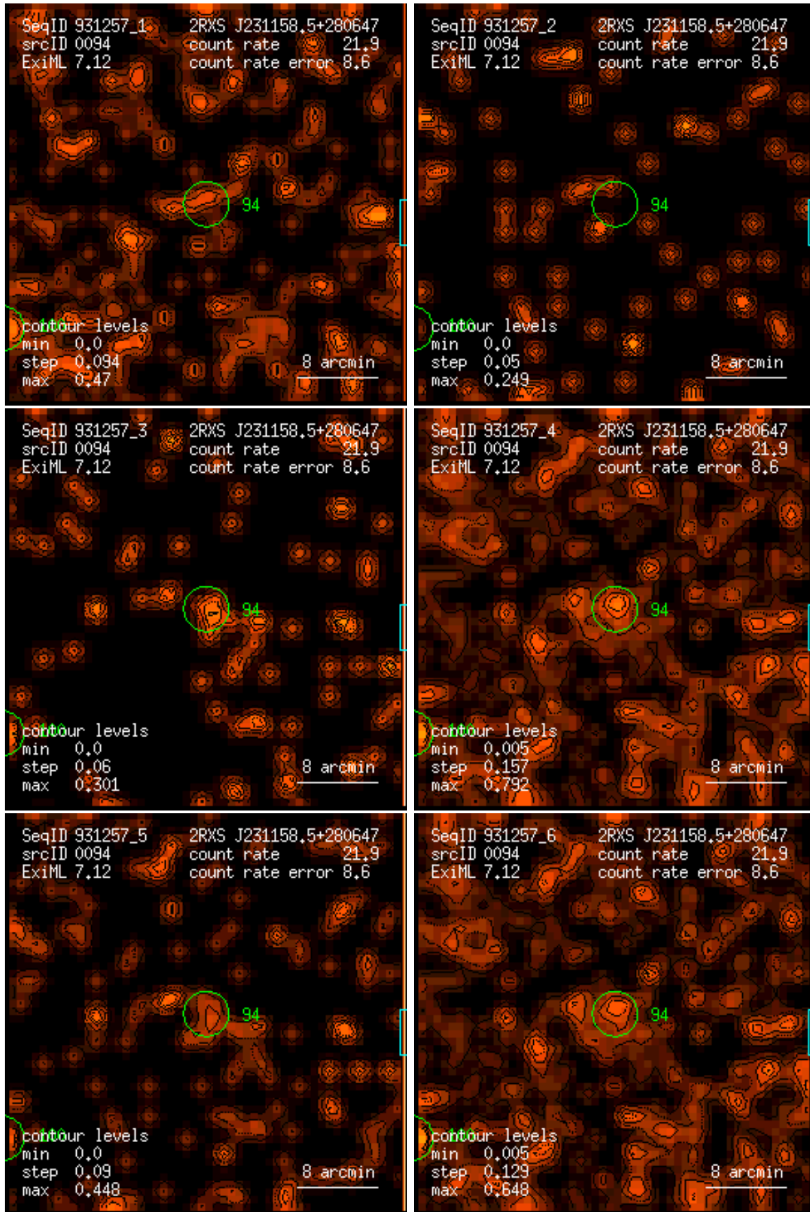
Figure 94: RASS 931257: detection 0094: band rate images, Gaussian filter: (1) PSPC channels 11 – 41, (2) 52 – 90, (3) 91 – 201, (4) 11 – 235, (5) 52 – 201, (6) 11 – 201. Broad band rates in counts/ks. Band rate contour levels in counts/ks/arcmin 2 .
