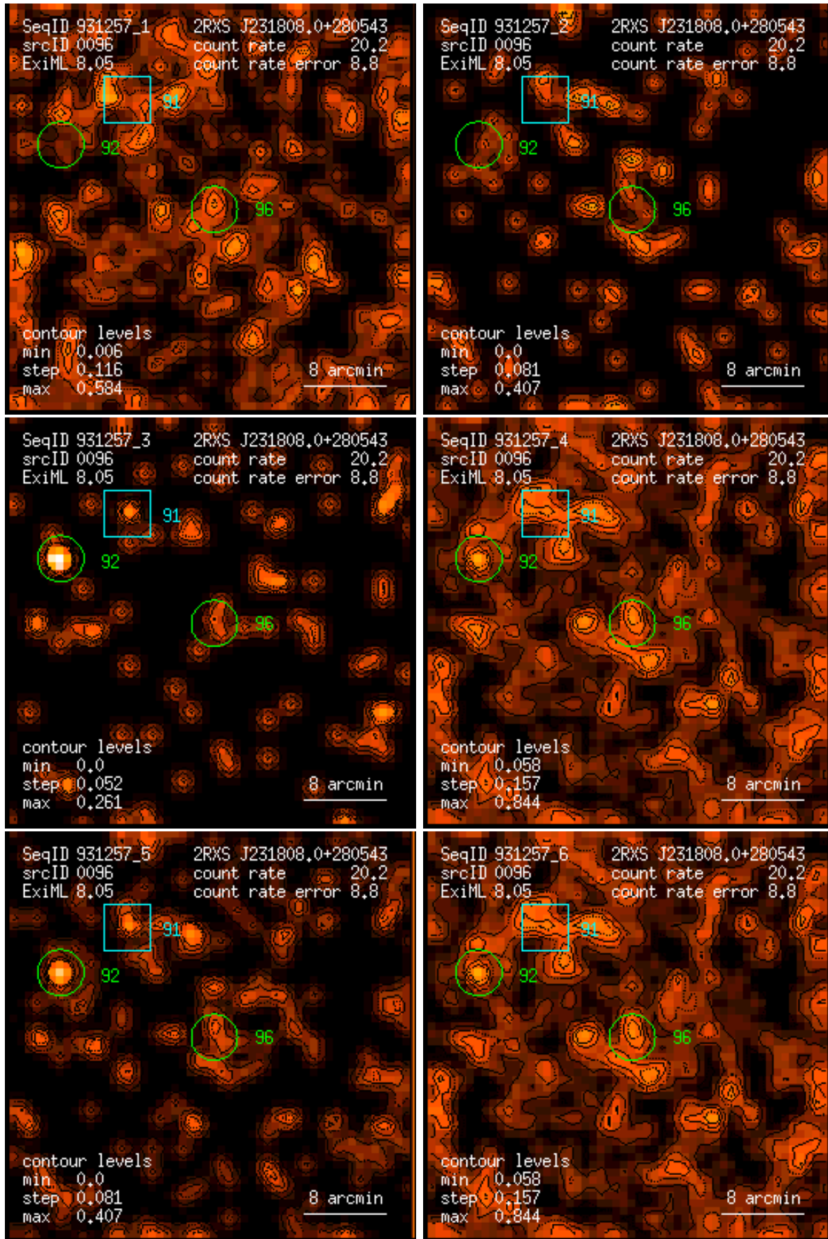
Figure 96: RASS 931257: detection 0096: band rate images, Gaussian filter: (1) PSPC channels 11 – 41, (2) 52 – 90, (3) 91 – 201, (4) 11 – 235, (5) 52 – 201, (6) 11 – 201. Broad band rates in counts/ks. Band rate contour levels in counts/ks/arcmin 2 .
