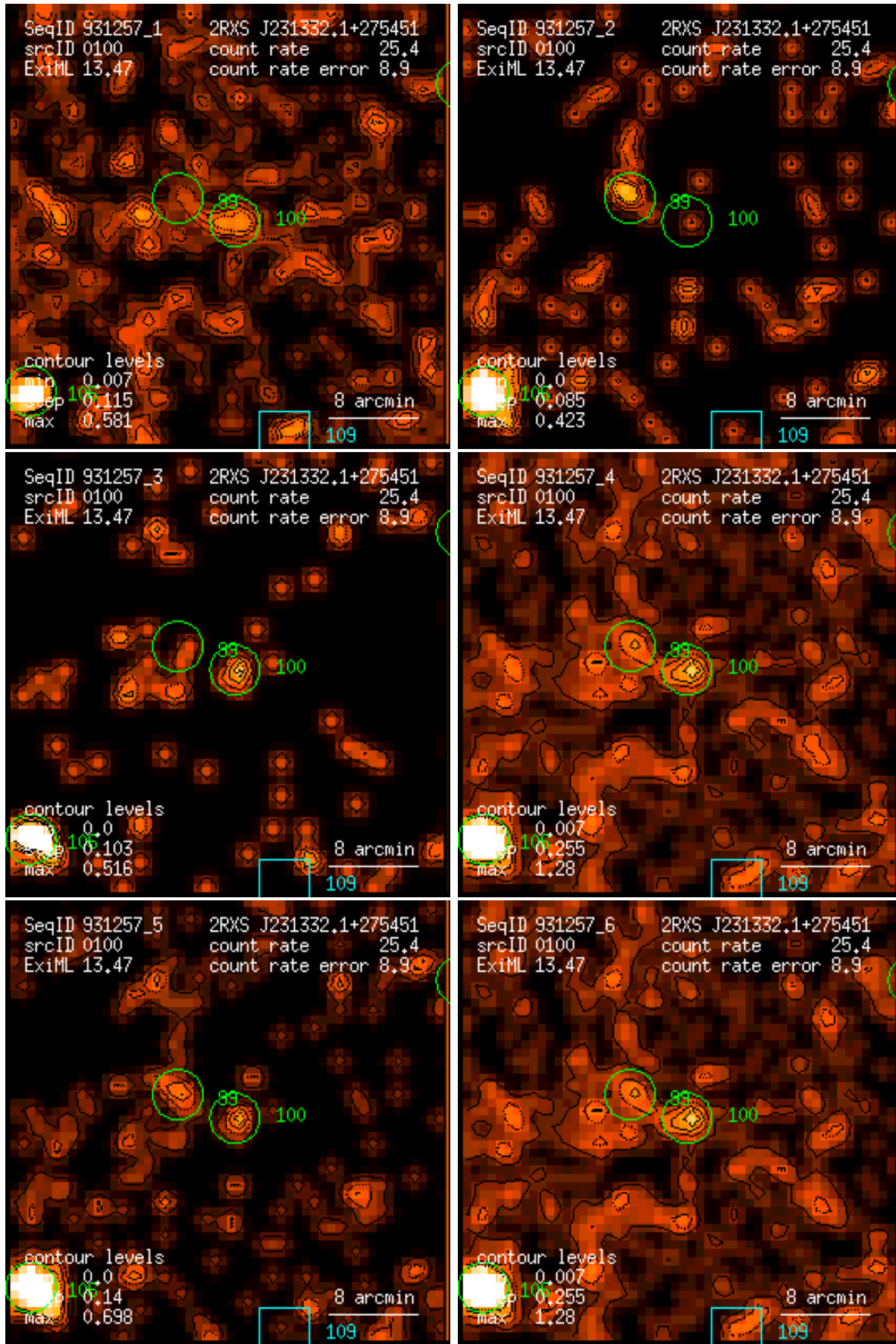
Figure 100: RASS 931257: detection 0100: band rate images, Gaussian filter: (1) PSPC channels 11 – 41, (2) 52 – 90, (3) 91 – 201, (4) 11 – 235, (5) 52 – 201, (6) 11 – 201. Broad band rates in counts/ks. Band rate contour levels in counts/ks/arcmin 2 .
