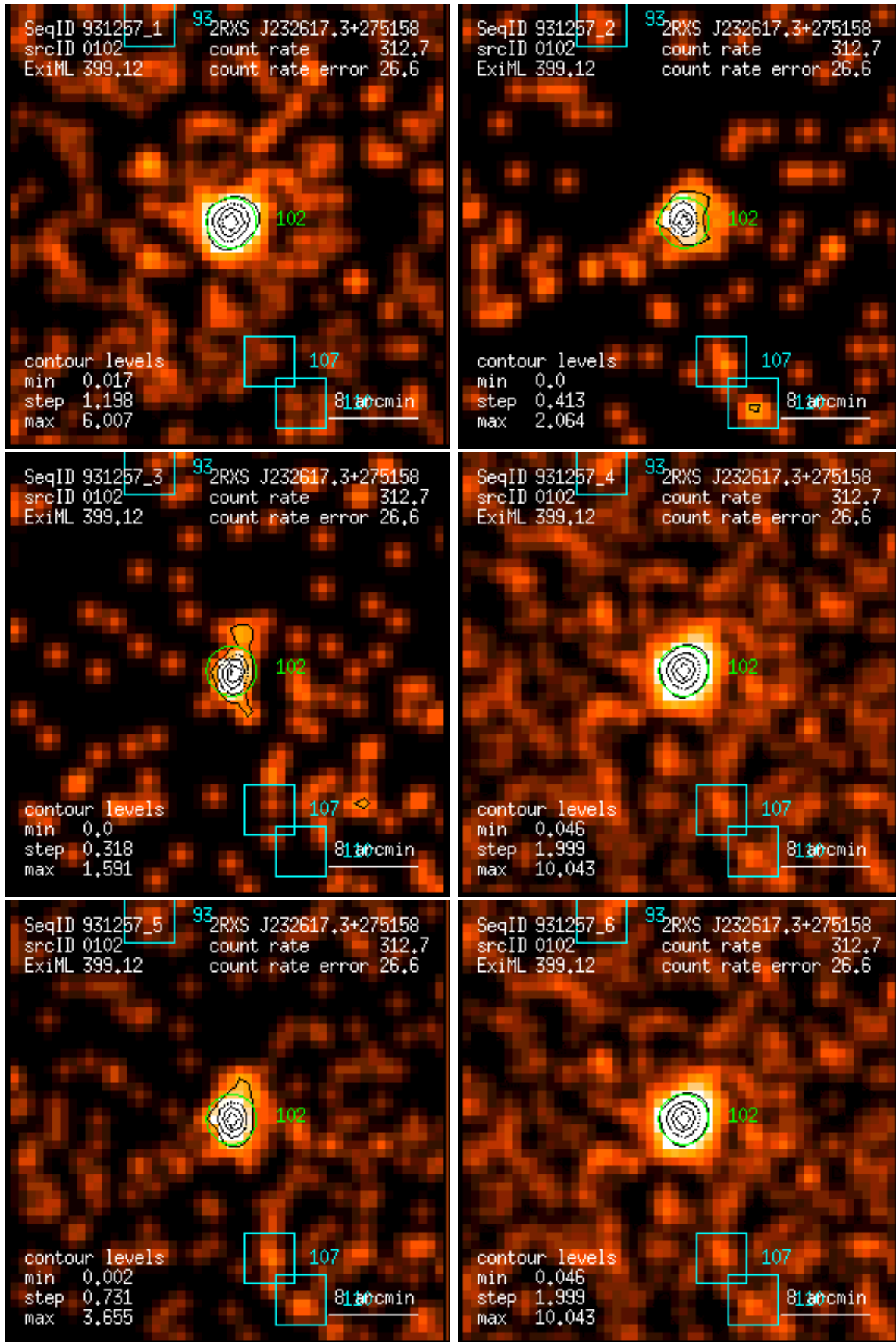
Figure 102: RASS 931257: detection 0102: band rate images, Gaussian filter: (1) PSPC channels 11 – 41, (2) 52 – 90, (3) 91 – 201, (4) 11 – 235, (5) 52 – 201, (6) 11 – 201. Broad band rates in counts/ks. Band rate contour levels in counts/ks/arcmin 2 .
