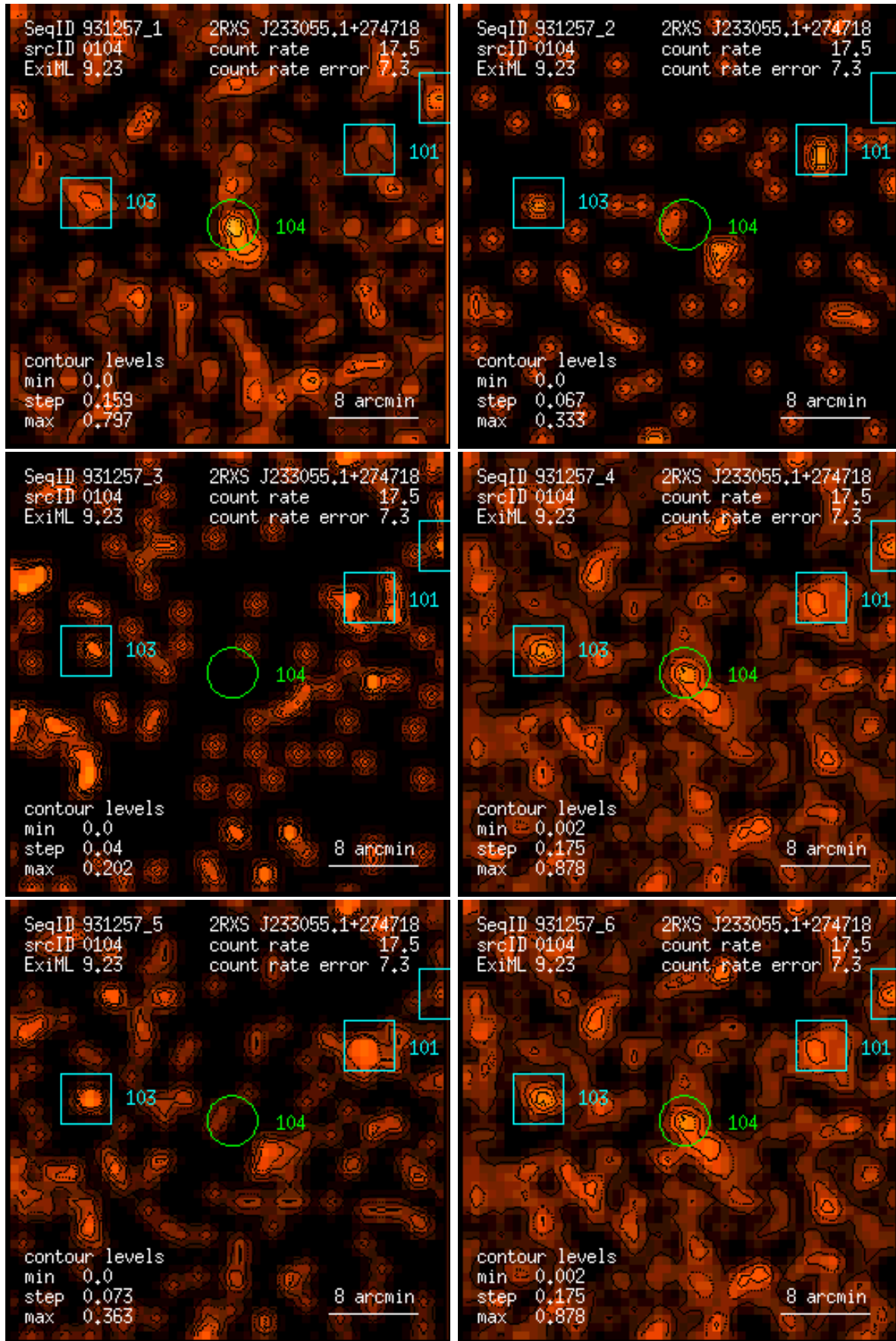
Figure 104: RASS 931257: detection 0104: band rate images, Gaussian filter: (1) PSPC channels 11 – 41, (2) 52 – 90, (3) 91 – 201, (4) 11 – 235, (5) 52 – 201, (6) 11 – 201. Broad band rates in counts/ks. Band rate contour levels in counts/ks/arcmin 2 .
